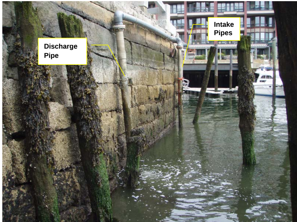
Figure 2: Intake and Discharge Pipes on Union Wharf Seawall
