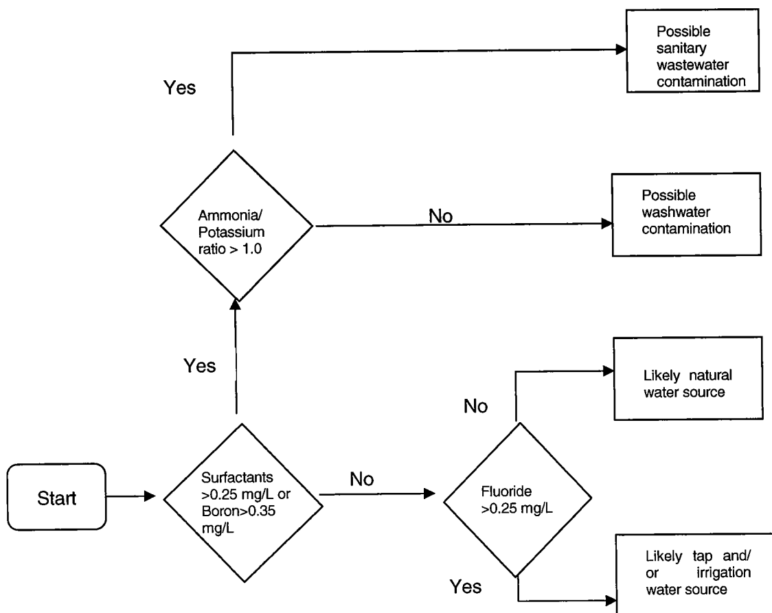
Figure 3: Flow Chart for Determining Likely Source of Discharge (Pitt, 2004)
