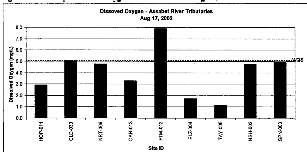
Figure 8: Tributary Dissolved Oxygen Concentrations – Aug 2002
