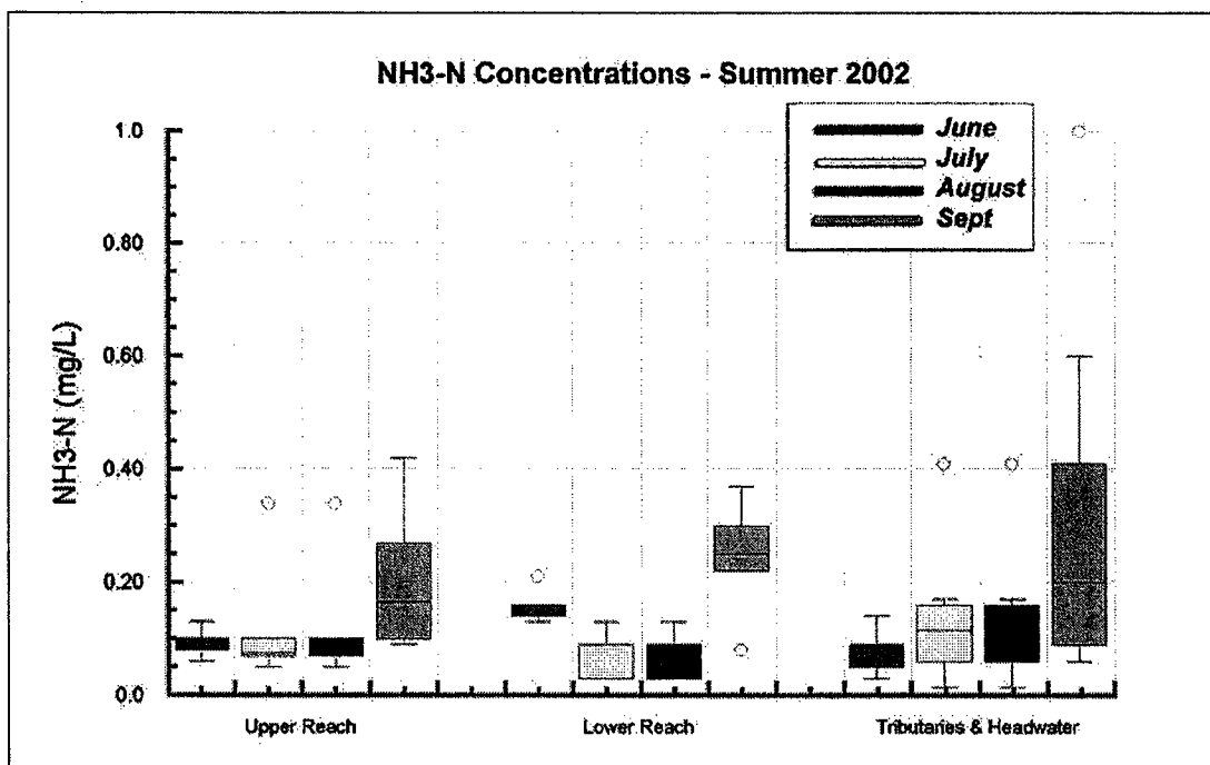
Figure 12: Median Ammonia Concentrations (2002)
