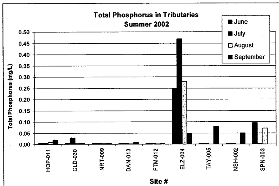
Figure 14: Total Phosphorus Concentrations in Tributaries
