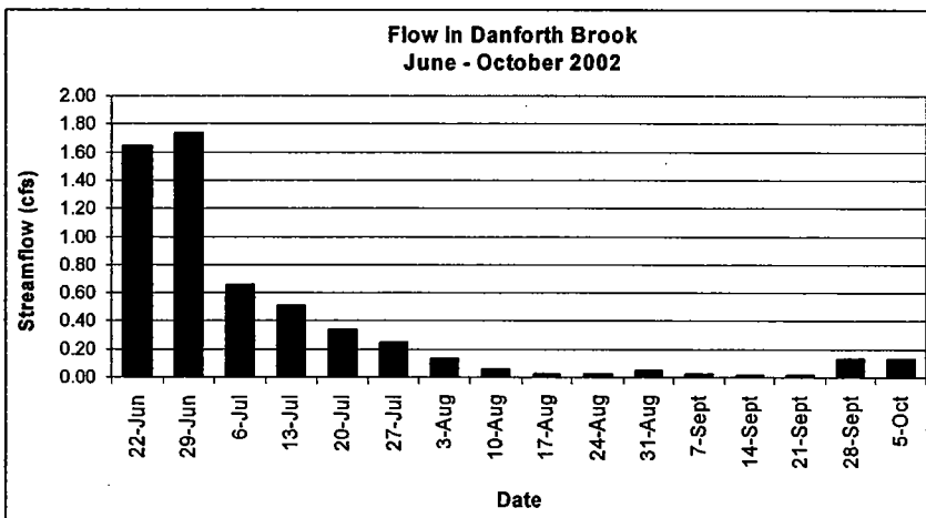
Figure 4: Flow in Danforth Brook - Summer 2002
