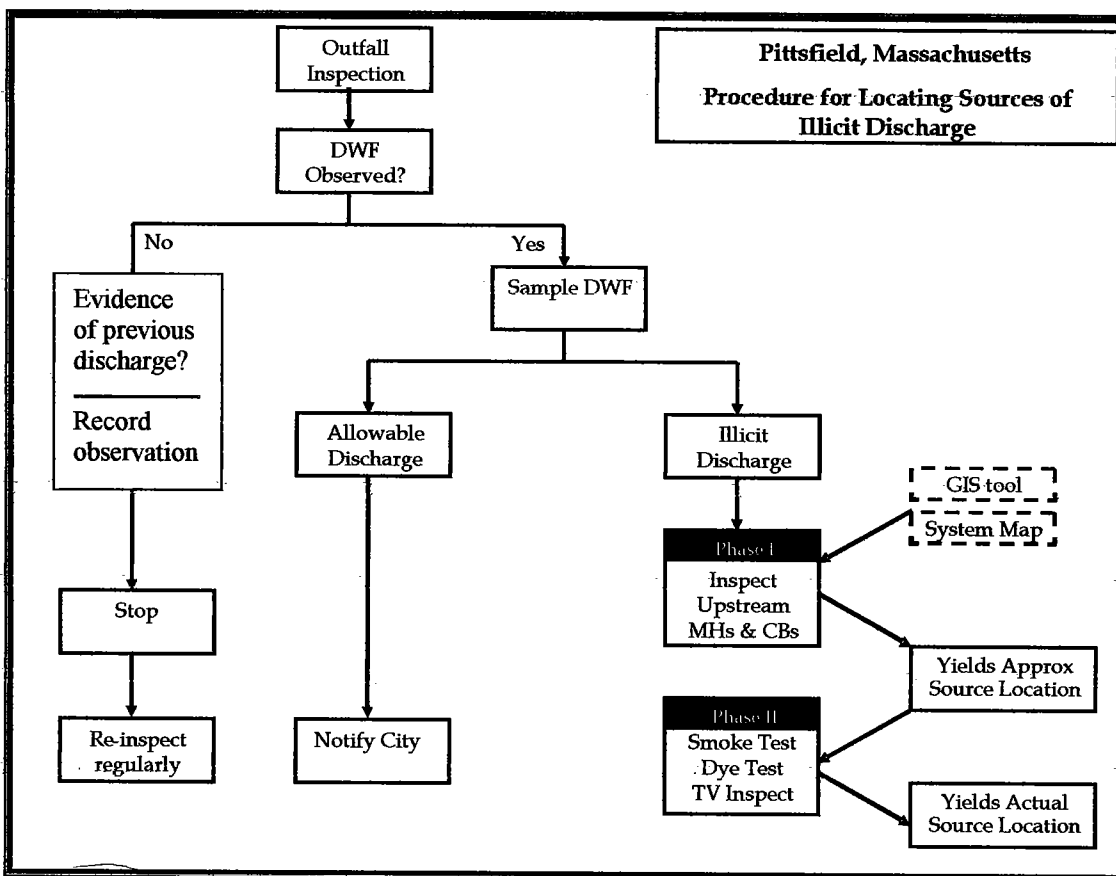
FIGURE 2.1 FLOW CHART SHOWING PROCESS OF IDENTIFYING ILLICIT DISCHARGE SOURCES
