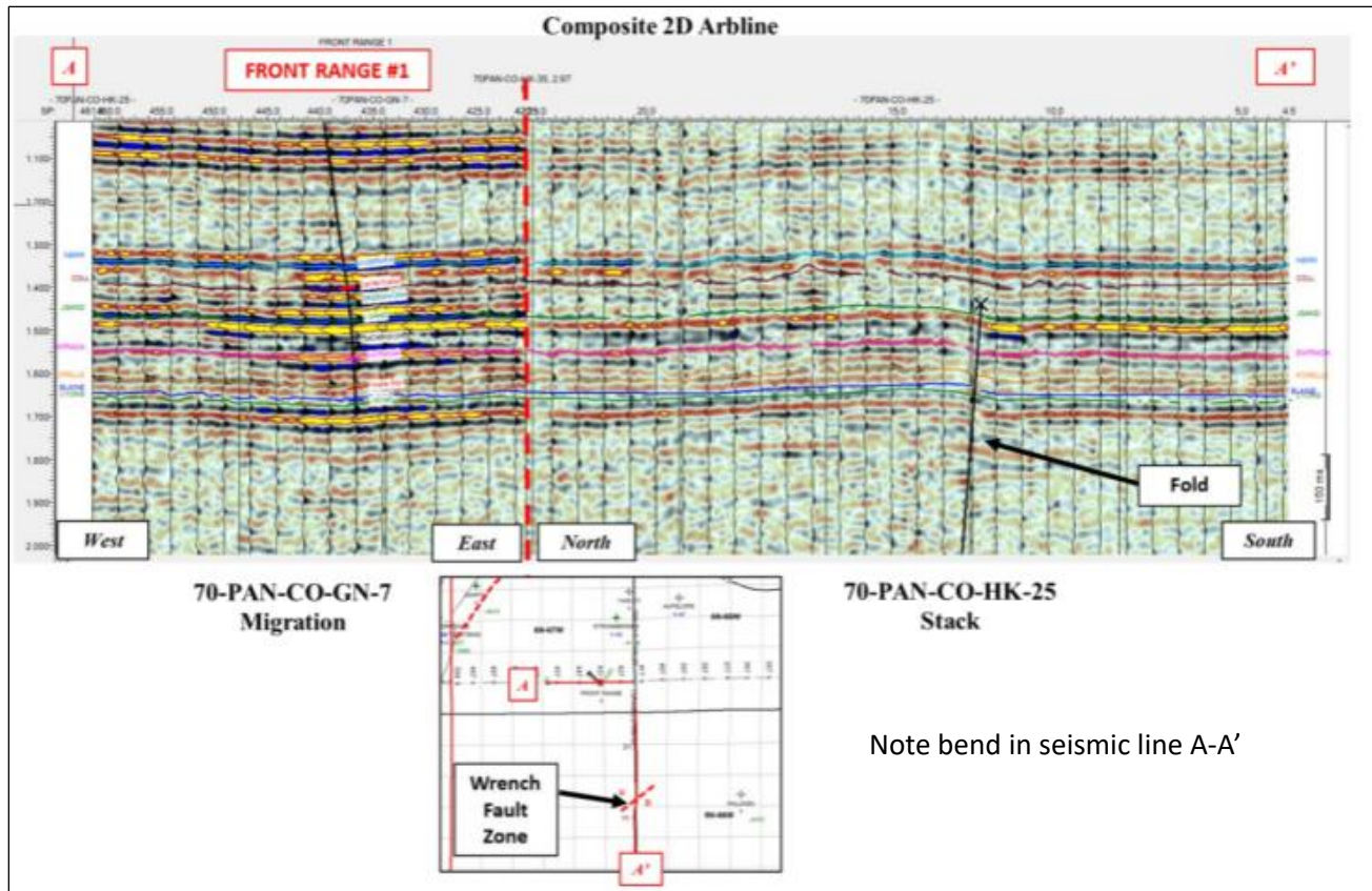
Figure 3. Composite 2D Seismic Line Across the Area of the Front Range 1-1 Well (CSS, 2024).
