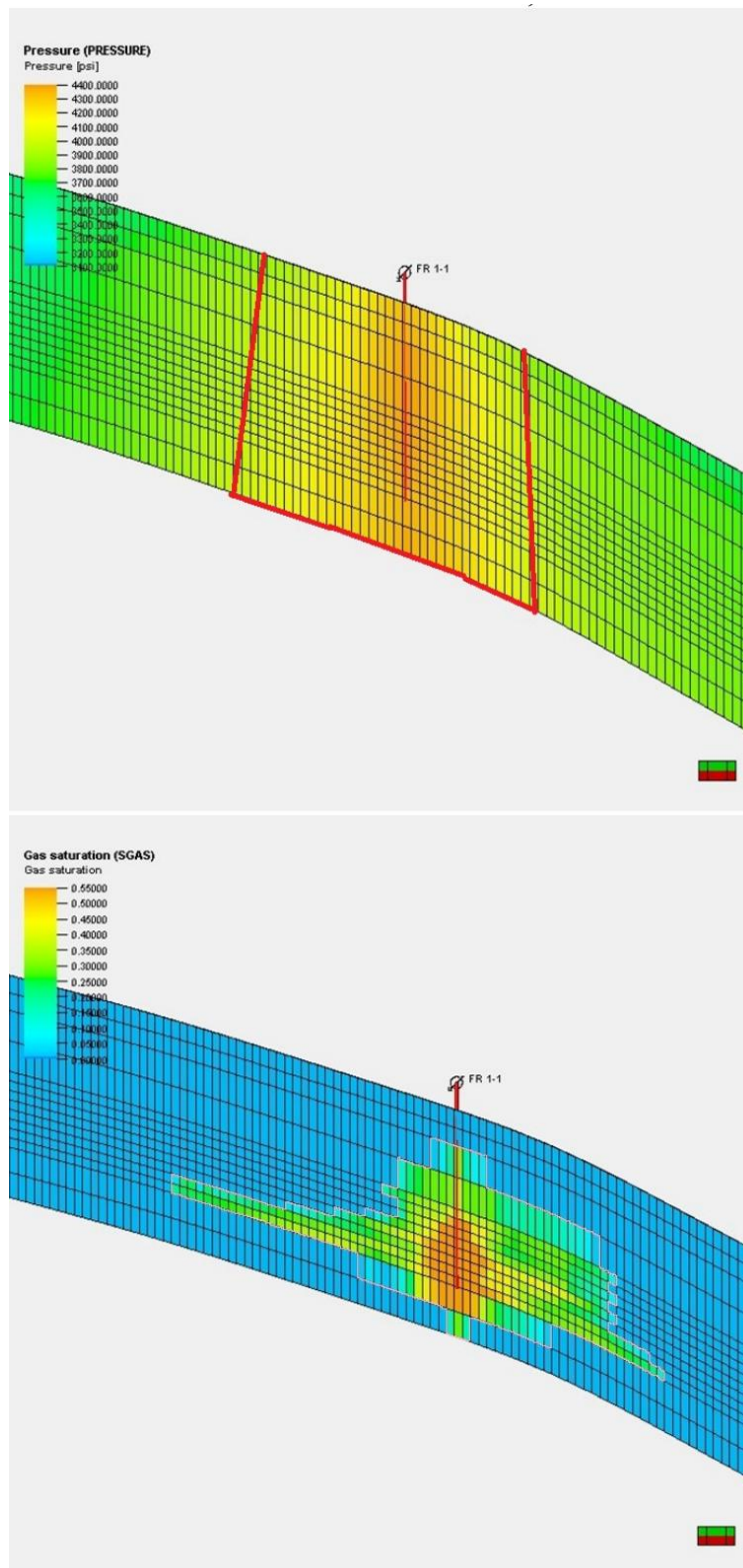
Figure 6. Delineation of Area of Review. Top Panel: Maximum extent of pressure front. Lower Panel: Maximum migration of CO 2 plume through modeled gas saturations. The AoR is a union of these parameters. (CSS, 2024)
