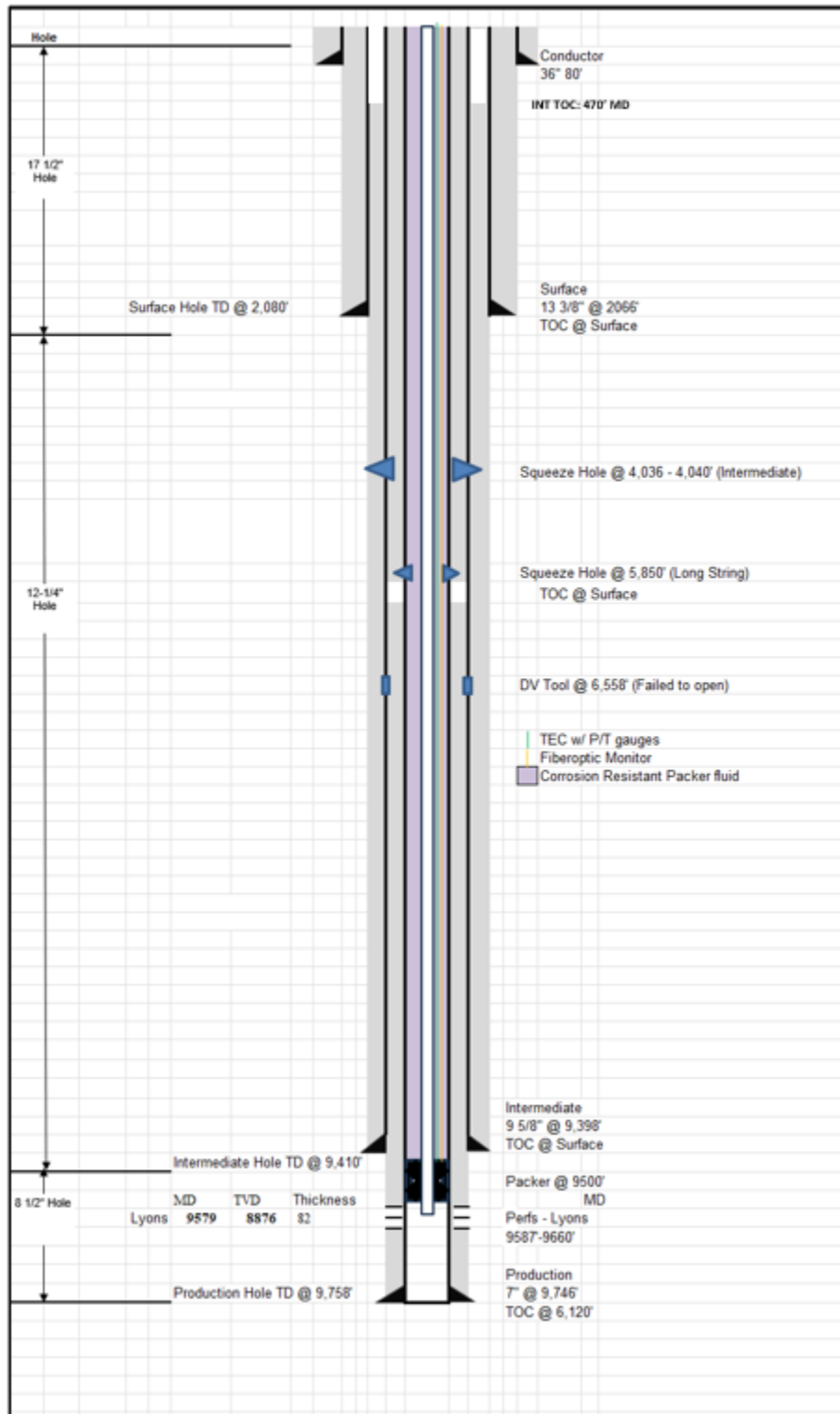
Figure 8b. Schematic of the Front Range 1-1 Injection Well. The diagram shows the current state of construction. Note the injection well is deviated and the measured depth and true vertical depth are different.
