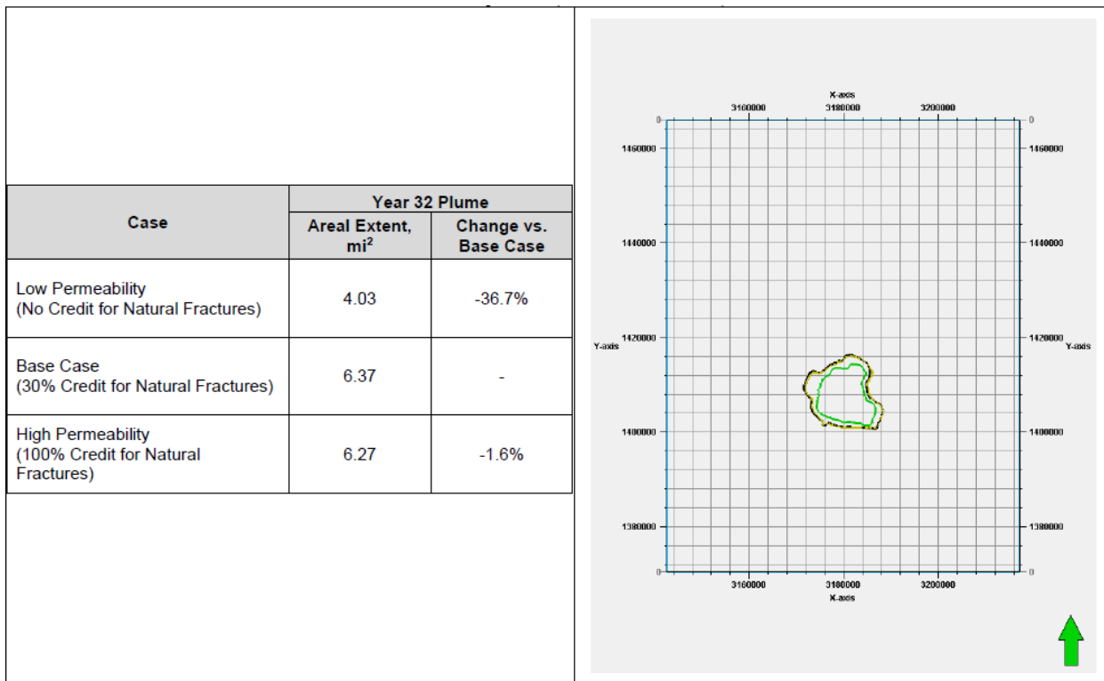
Figure 7. Right: Areal Extent of Year 32 Plumes for Low Permeability Case (Green Line), Base (Black Line), and High Permeability Cases (Yellow-Green Line).
