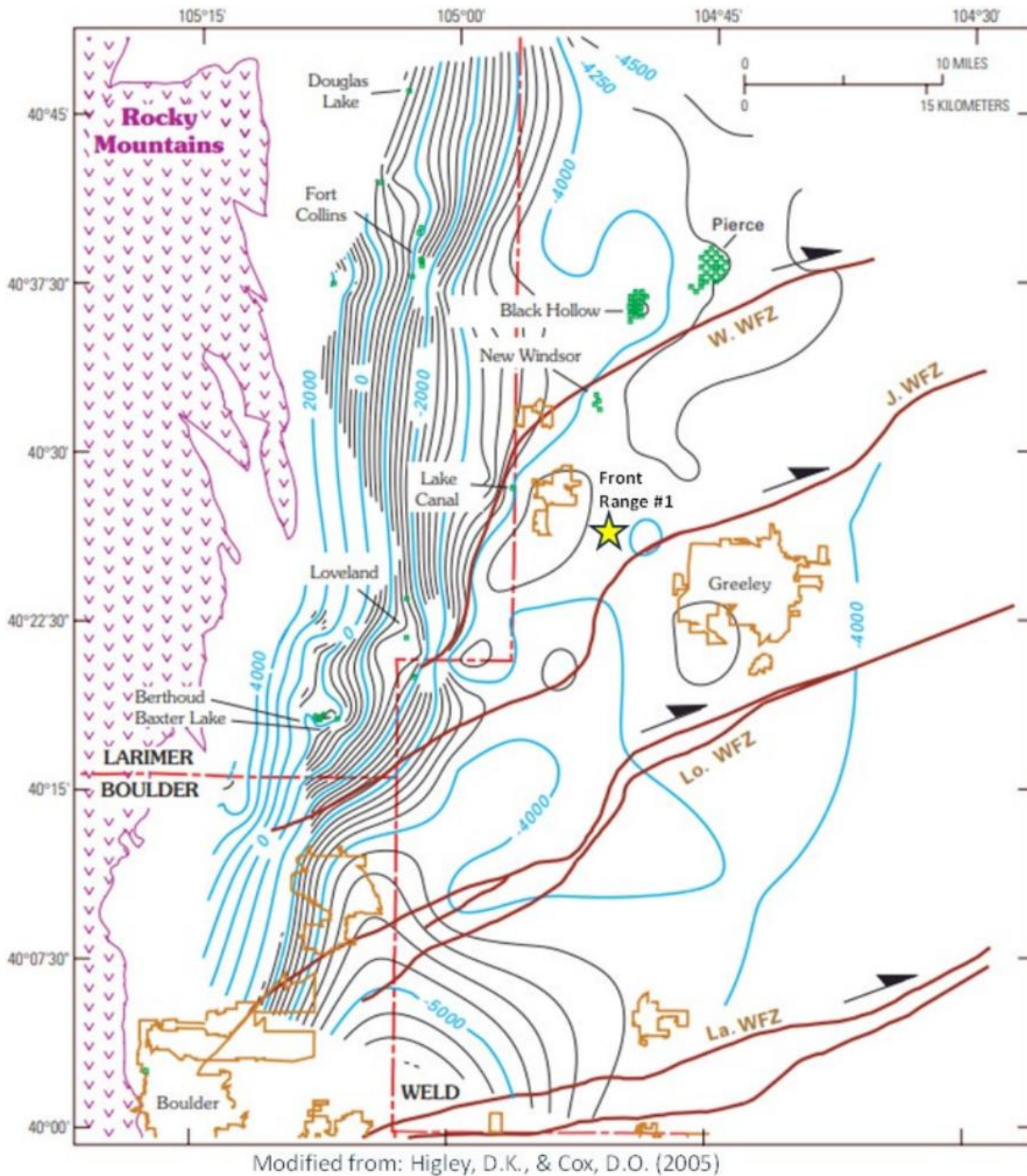
Figure 2. Map Showing Location of Wrench Faults in the Denver Basin. Labeled wrench faults at Windsor (W. WFZ), Johnstown (J. WFZ), Longmont (Lo. WFZ), and Lafayette (La. WFZ) arrows indicate direction of lateral movement. (CSS, 2024)
