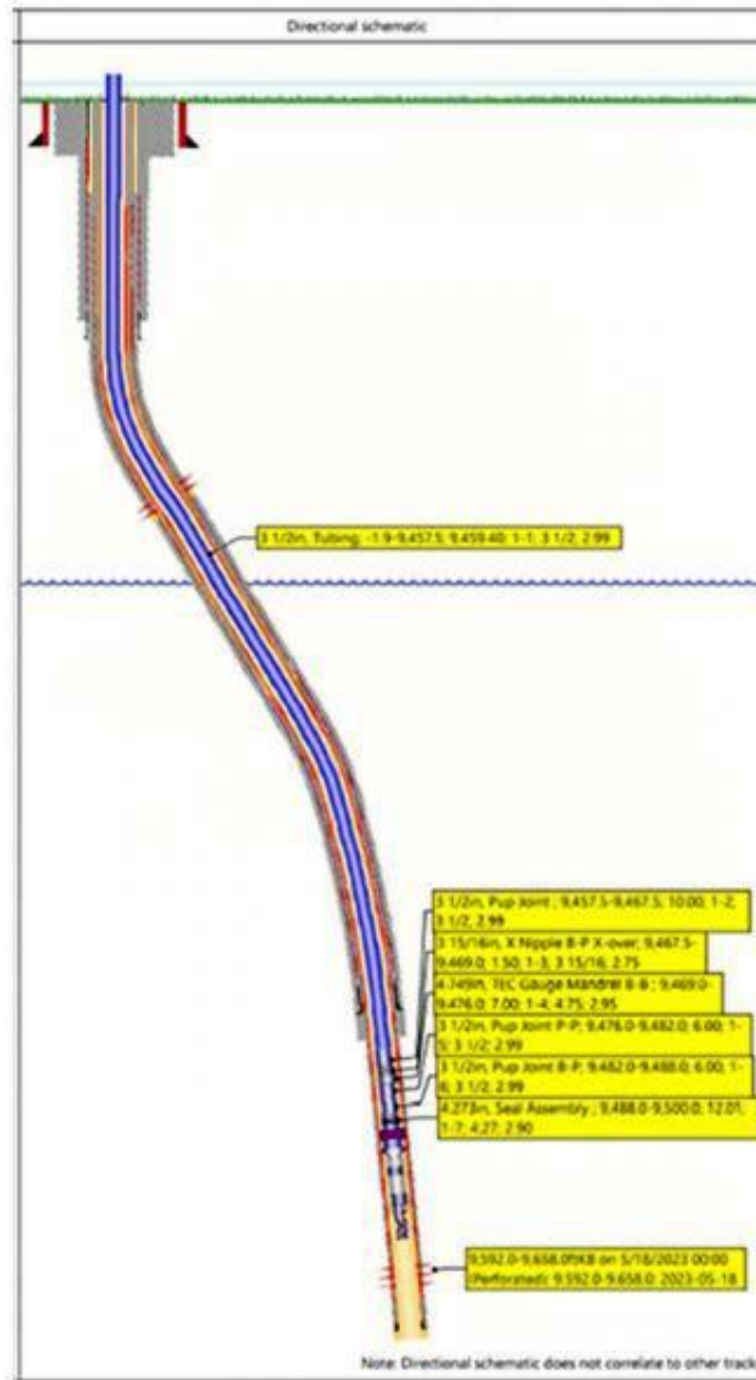
Figure 8a: Directional Wellbore Schematic for Front Range 1-1
