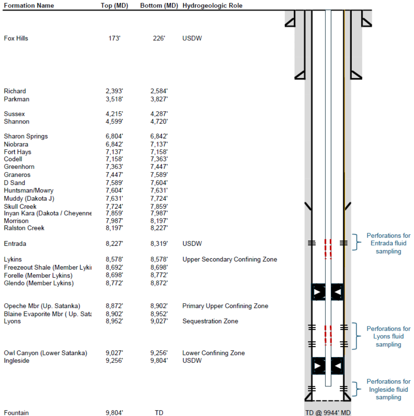
Figure 9. Wellbore schematic for the Front Range 2-1, including internal mechanisms for fluid sampling of the injection zone and the adjacent USDWs.
