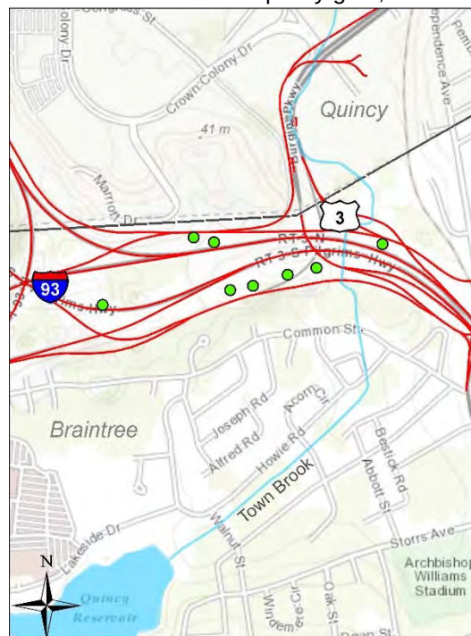
Project Limits and BMP Locations
