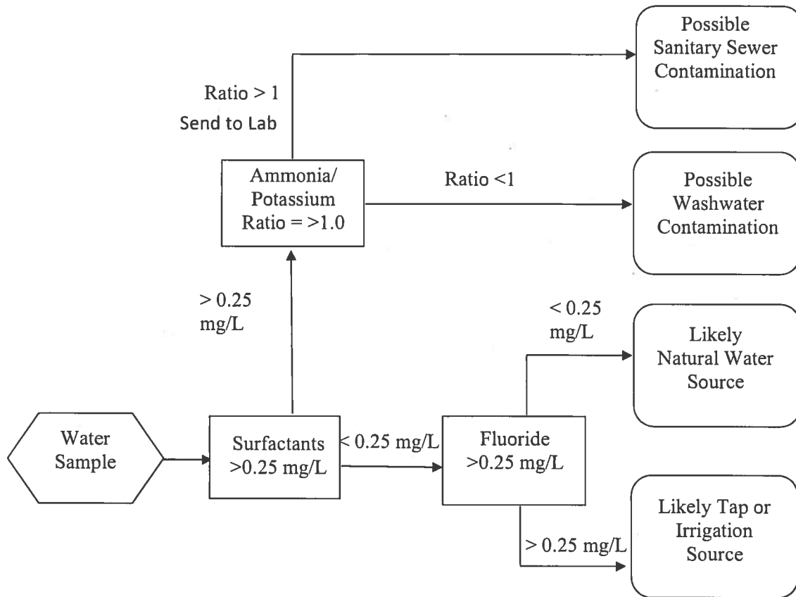
Figure 2 Illicit Discharge Flow Diagram
