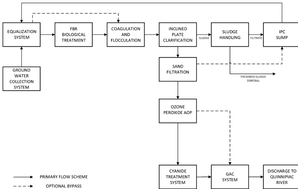
Figure 2-1 Primary Flow Scheme
