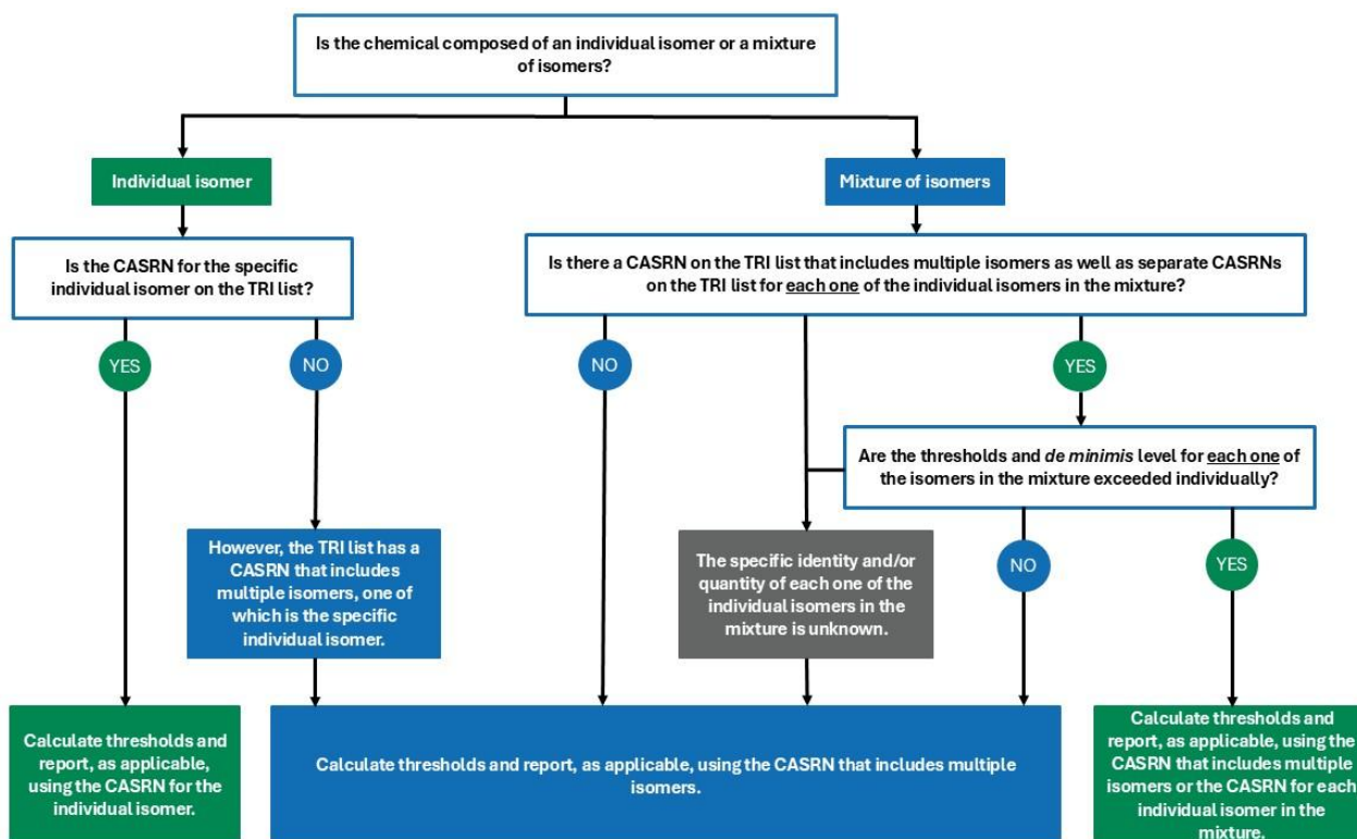
Figure 5. Flow Diagram for Determining Thresholds for CASRN's That Include Multiple Isomers of a Chemical
