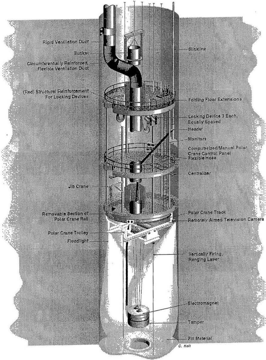
Figure G2B-1 Multi-Deck Stage Illustrating Dynamic Compaction
