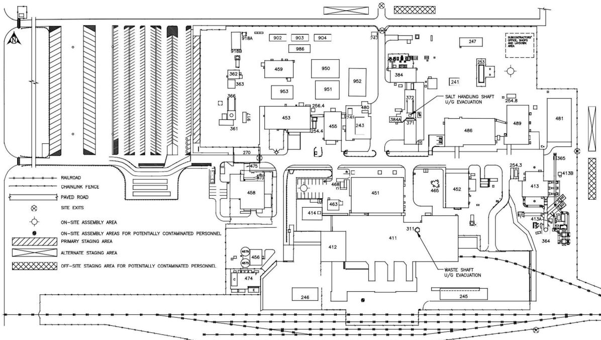
Figure D-1 WIPP Surface Structures
