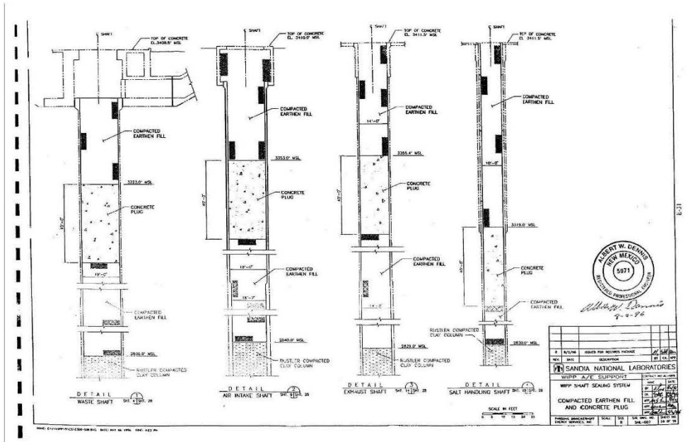
Compacted Earthen Fill and Concrete Plug
