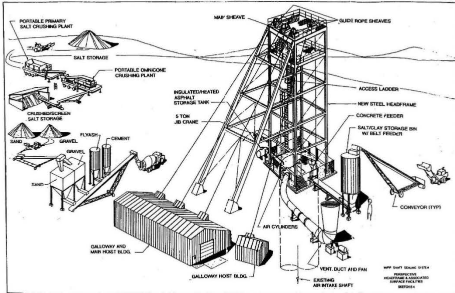
WPP Shaft Sealing System Typical Headframe and Associated Surface Facilities
