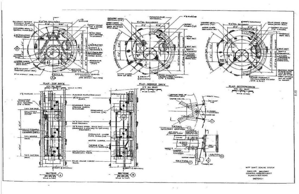
WIPP Shaft Sealing System Smaller Galloway Genral Arrangement Plans and Sections
