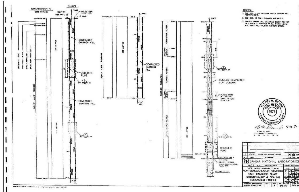
Near-Surface / Ruster Formations Salt Handling Shaft Stratigraphy and Sealing Subsystem Profile
