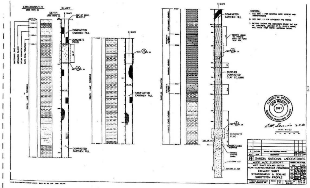
Near-Surface / Rustler Formations Exhaust Shaft Stratigraphy and Sealing Subsystem Profile
