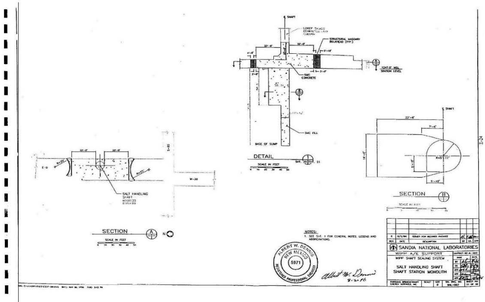
Salt Handling Shaft Shaft Station Monolith
