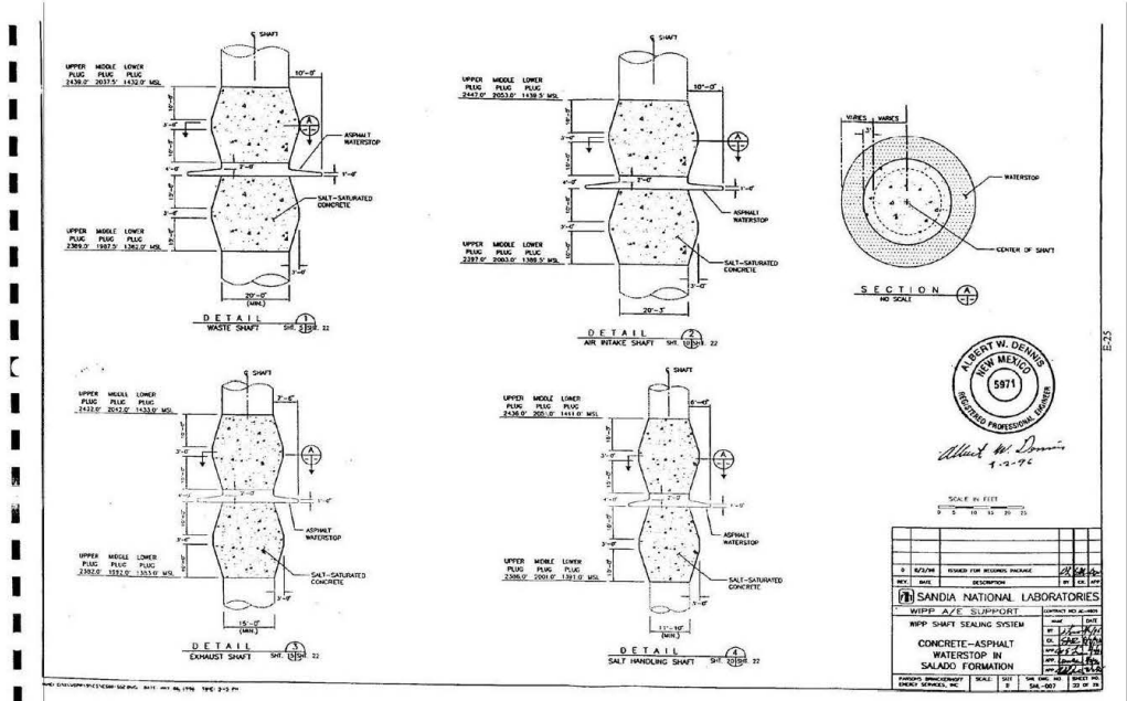
Concrete-Asphalt Water Stop in Salado Formation
