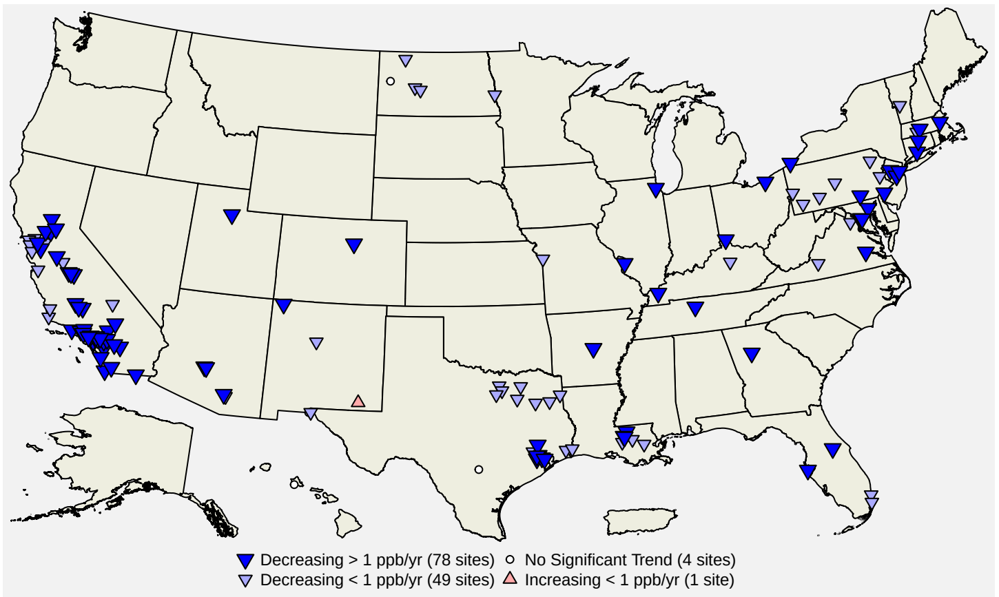
Figure 8: Site-level trends in 1-hour NO 2 design values based on data from 2000 through 2025. Source: AQS, trends computed using R statistical software.
