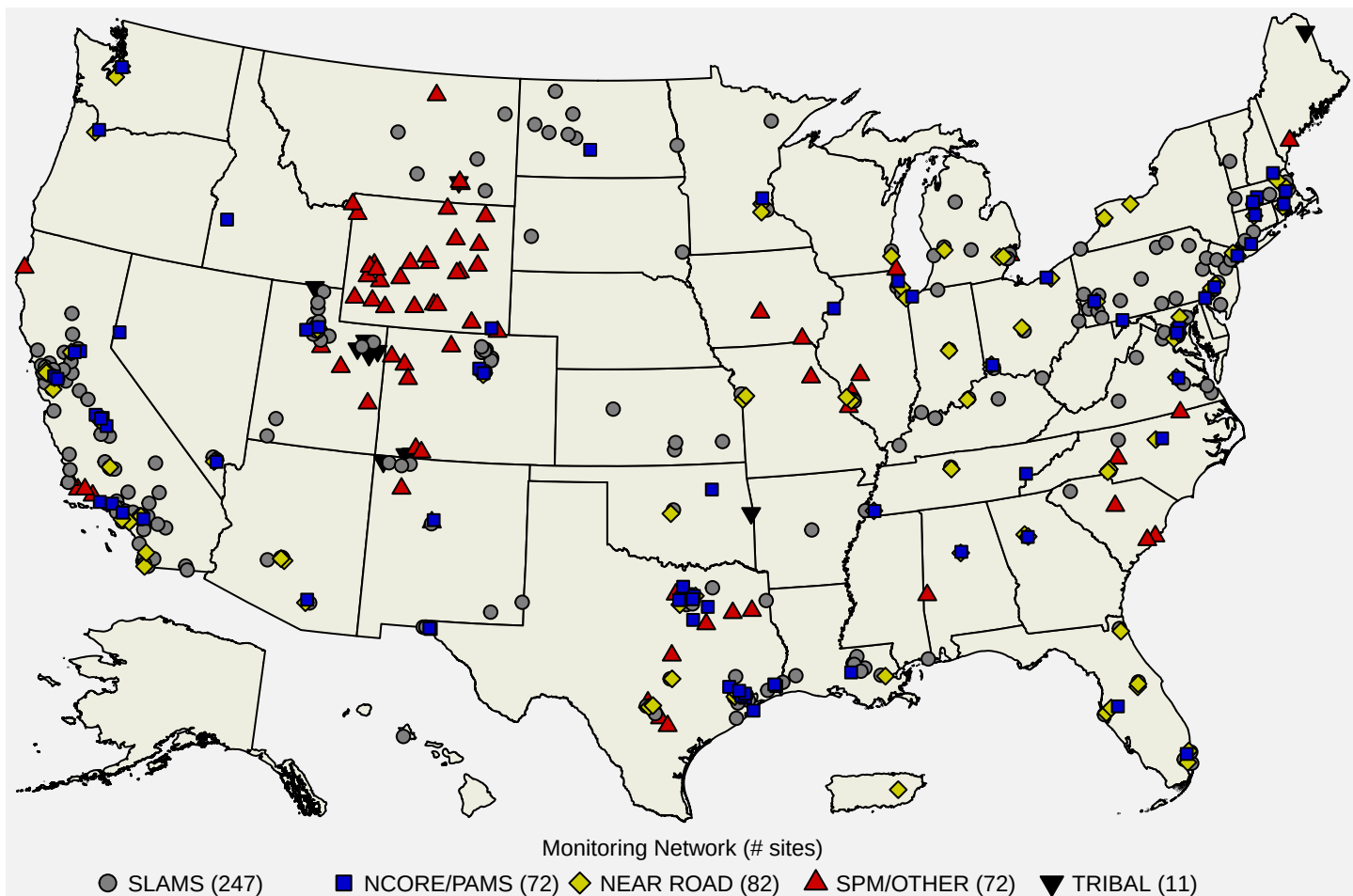
Figure 4: Map of U.S. NO 2 monitoring sites reporting data to the EPA during the 2023-2025 period. Source: AQS .
