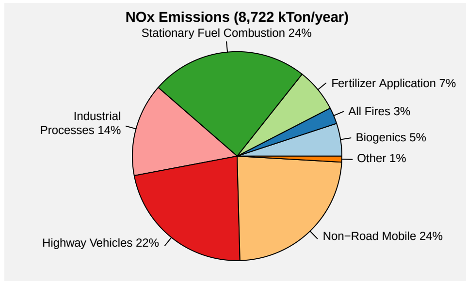
Figure 1. U.S. NO x emissions by sector. Source: 2023 NEI.
