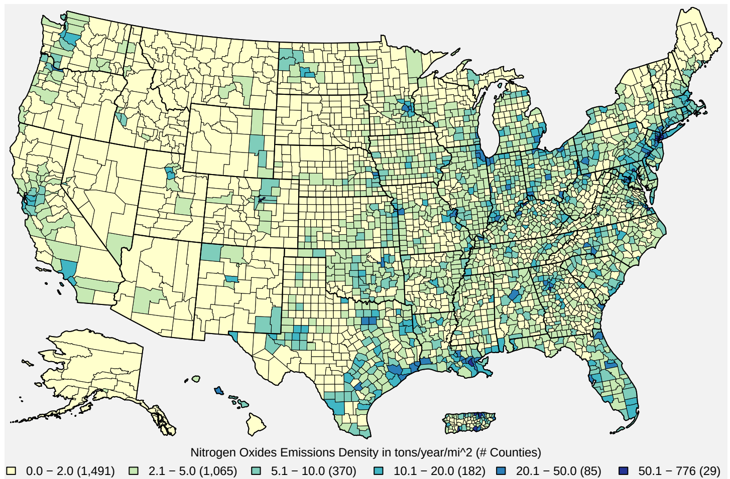
Figure 2. U.S. county-level NO x emissions density estimates in tons/year/mi 2 . Source: 2023 NEI
