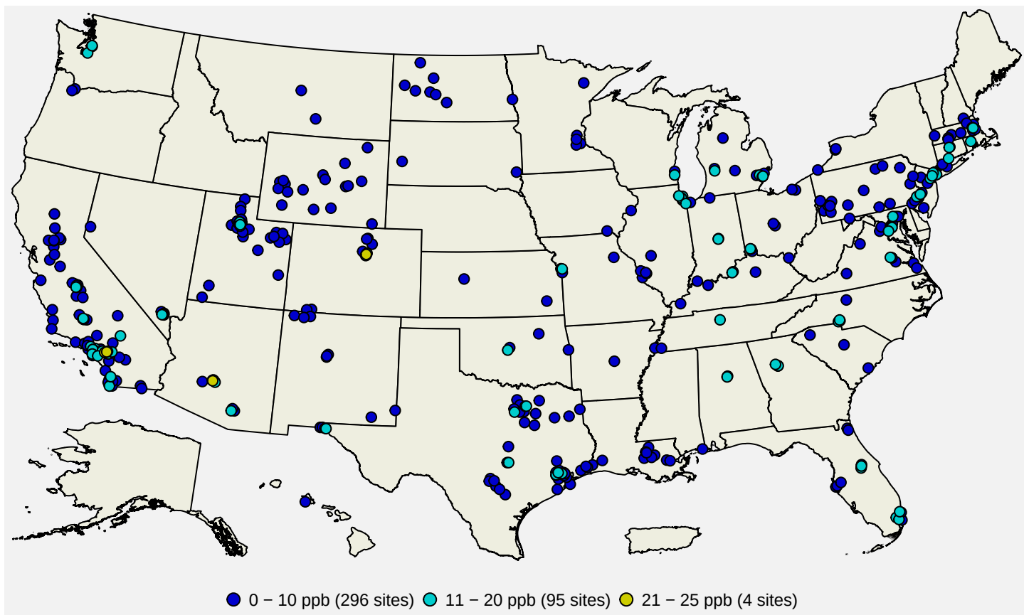
Figure 5: Annual NO 2 design values in ppb based on data from 2025. Source: AQS .
