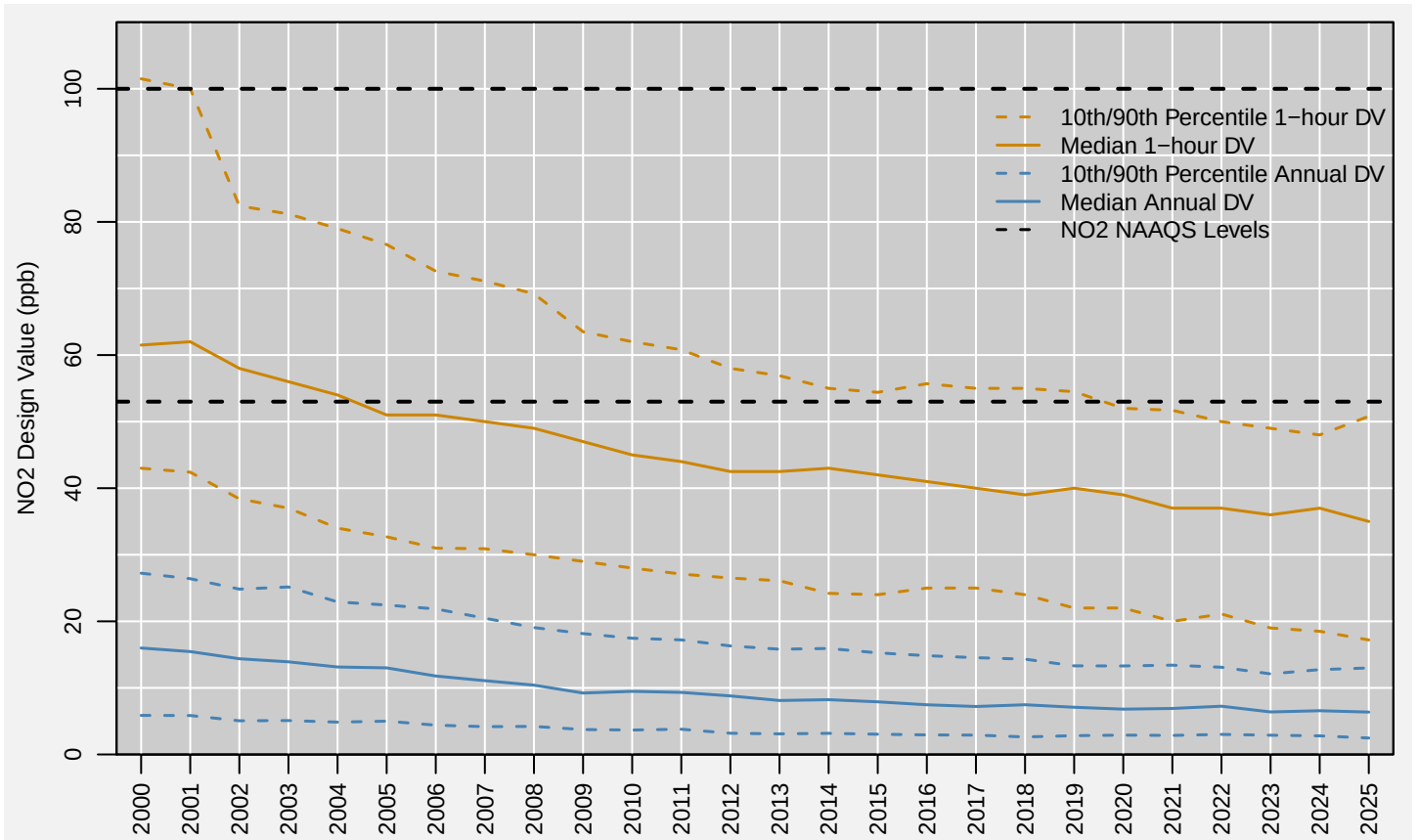
Figure 9: National trends in NO 2 design values in ppb, 2000 to 2025. Source: AQS.
