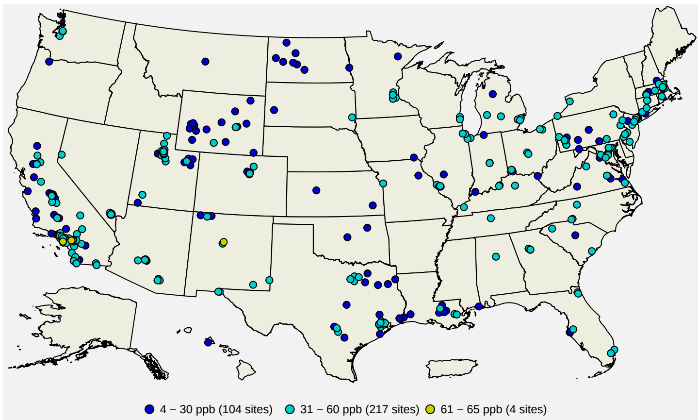
Figure 6: 1-hour NO 2 design values in ppb for the 2023-2025 period. Source: AQS .
