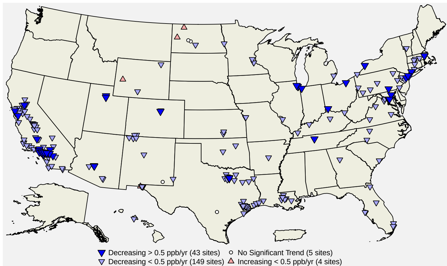
Figure 7: Site-level trends in annual NO 2 design values based on data from 2000 through 2025. Source: AQS, trends computed using R statistical software.
