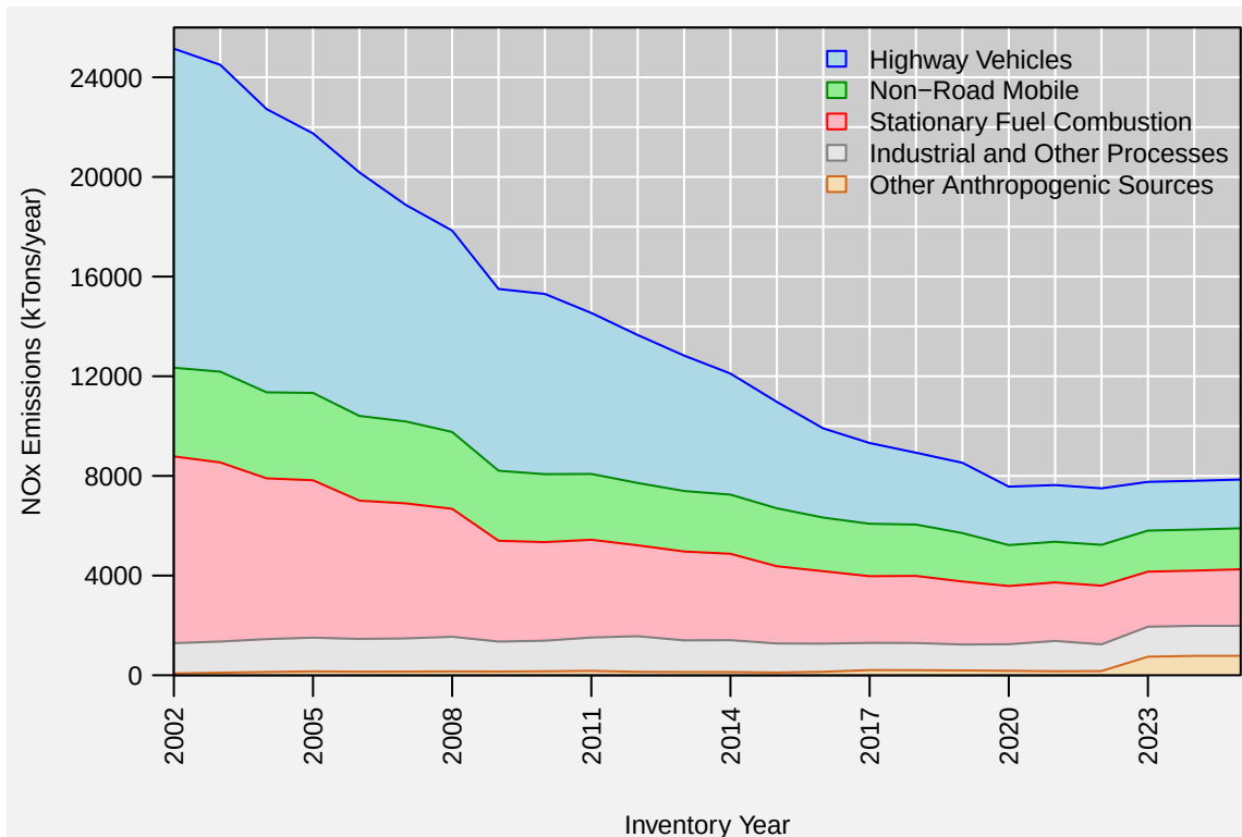
Figure 3. U.S. anthropogenic NO x emissions trend, 2002-2025. Source: EPA's Air Pollutant Emissions Trends Data
