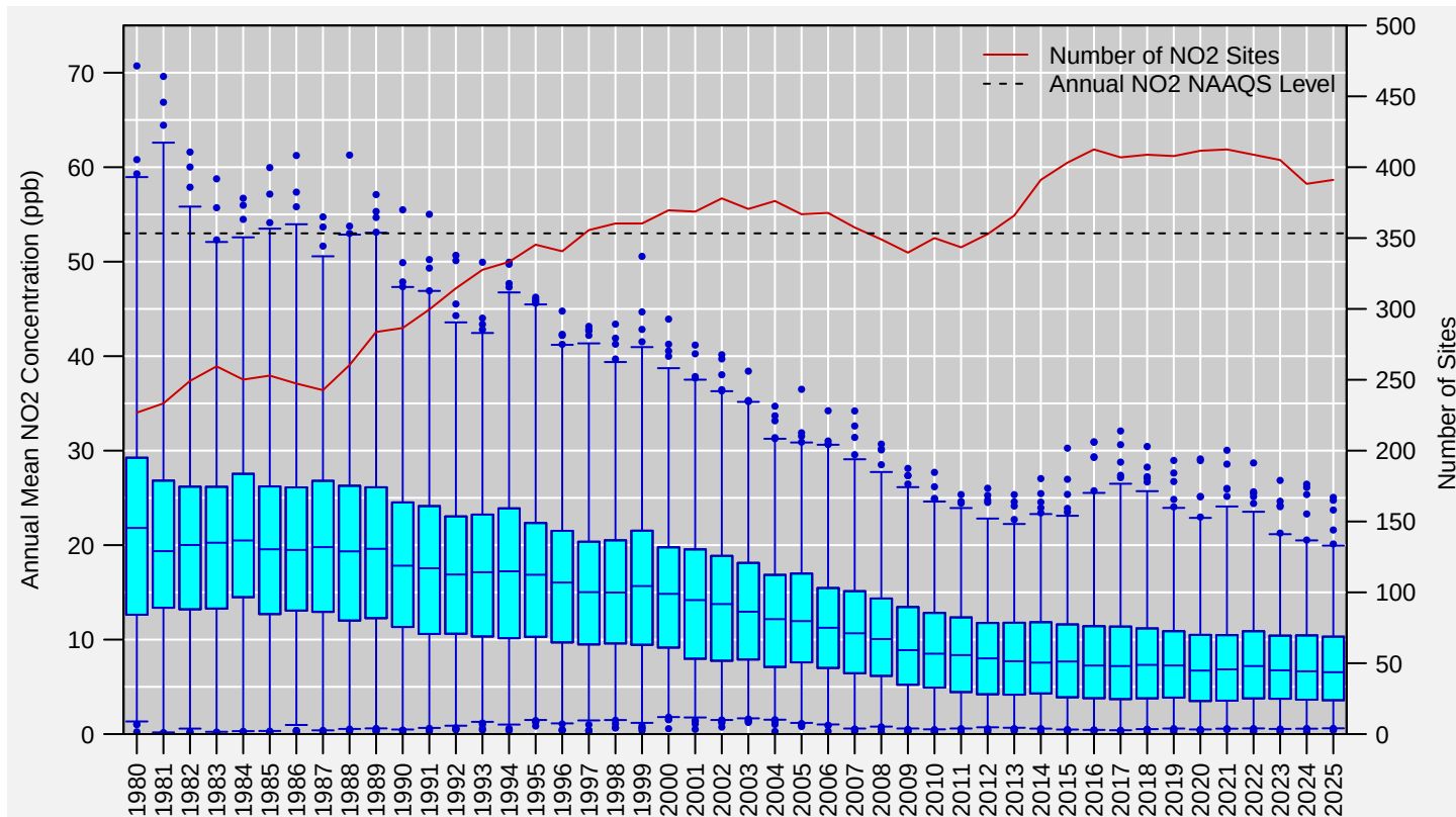
Figure 10: Distribution of annual mean NO 2 concentrations measured at U.S. monitoring sites, 1980 to 2025. Boxes represent the median and interquartile range, whiskers extend to the 1st and 99th percentiles, and values outside this range are shown as circles. The red line shows the number of NO 2 monitoring sites reporting data to EPA in each year. Source: AQS.
