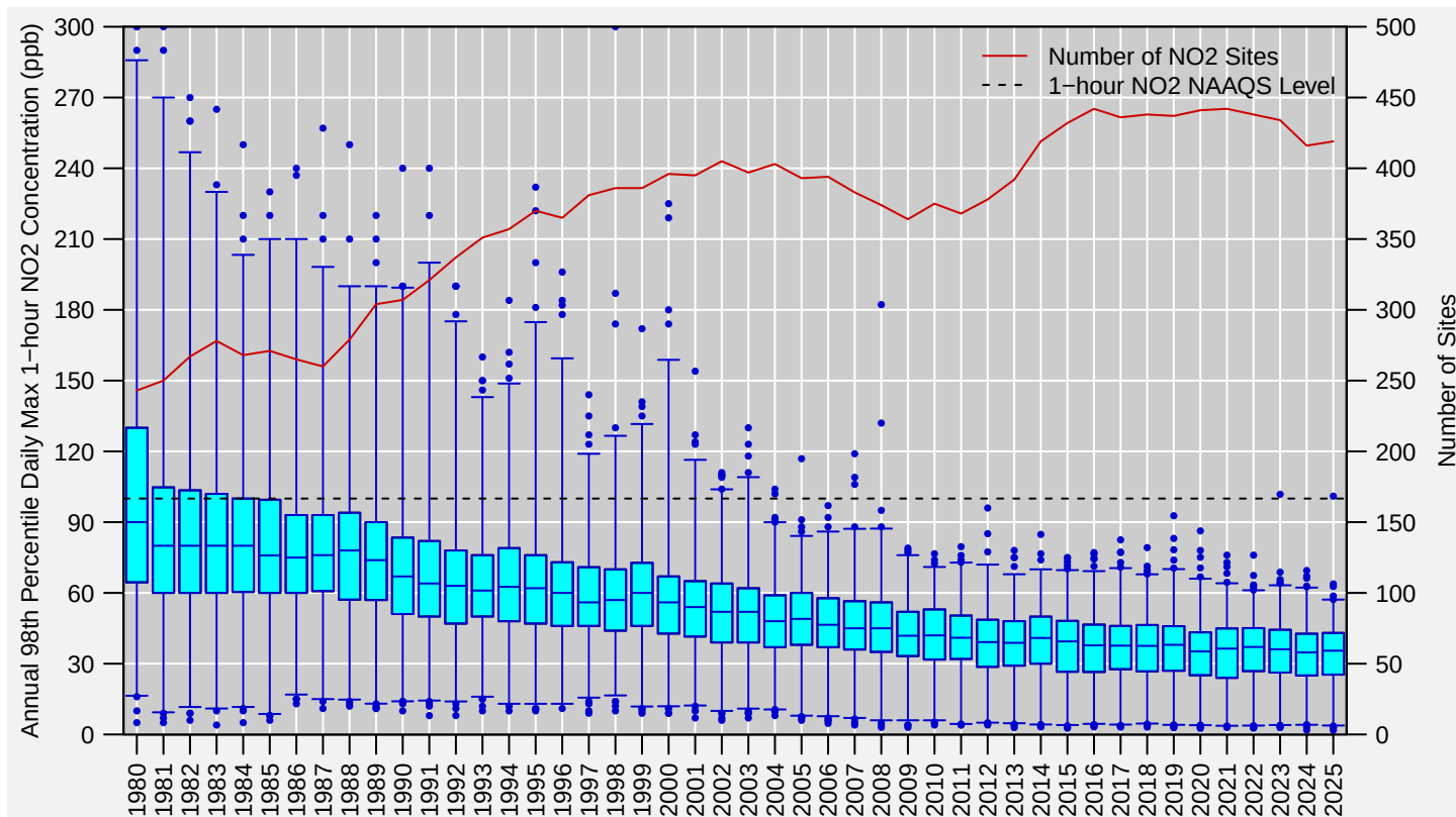
Figure 11: Distribution of annual 98th percentile MDA1 NO 2 concentrations measured at U.S. monitoring sites, 1980 to 2025. Boxes represent the median and interquartile range, whiskers extend to the 1st and 99th percentiles, and values outside this range are shown as circles. The red line shows the number of NO 2 monitoring sites reporting data to EPA in each year. Source: AQS.
