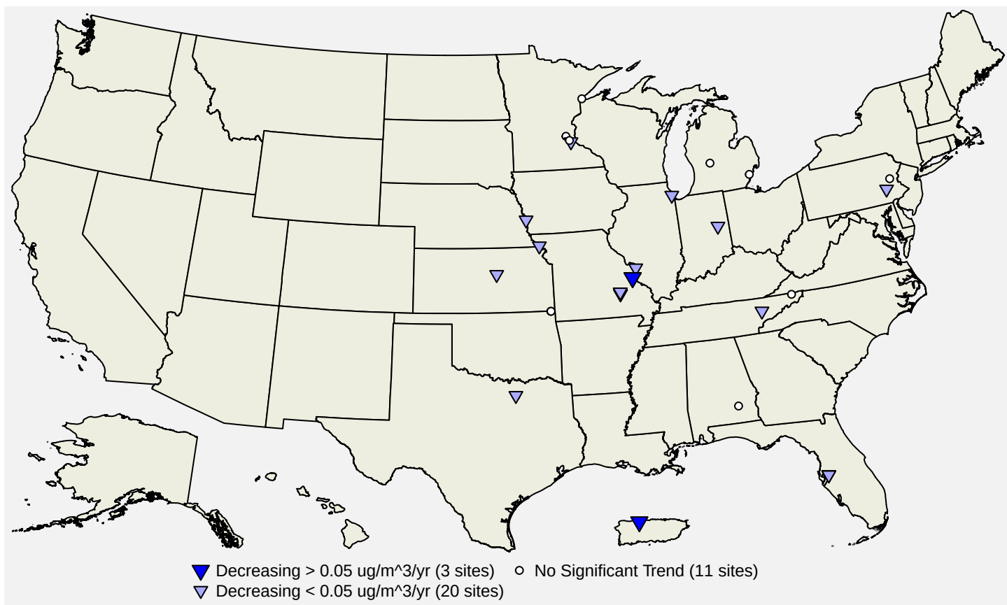
Figure 7: Site-level trends in Pb design values based on data from 2010 through 2025. Source: AQS, trends computed using R statistical software.
