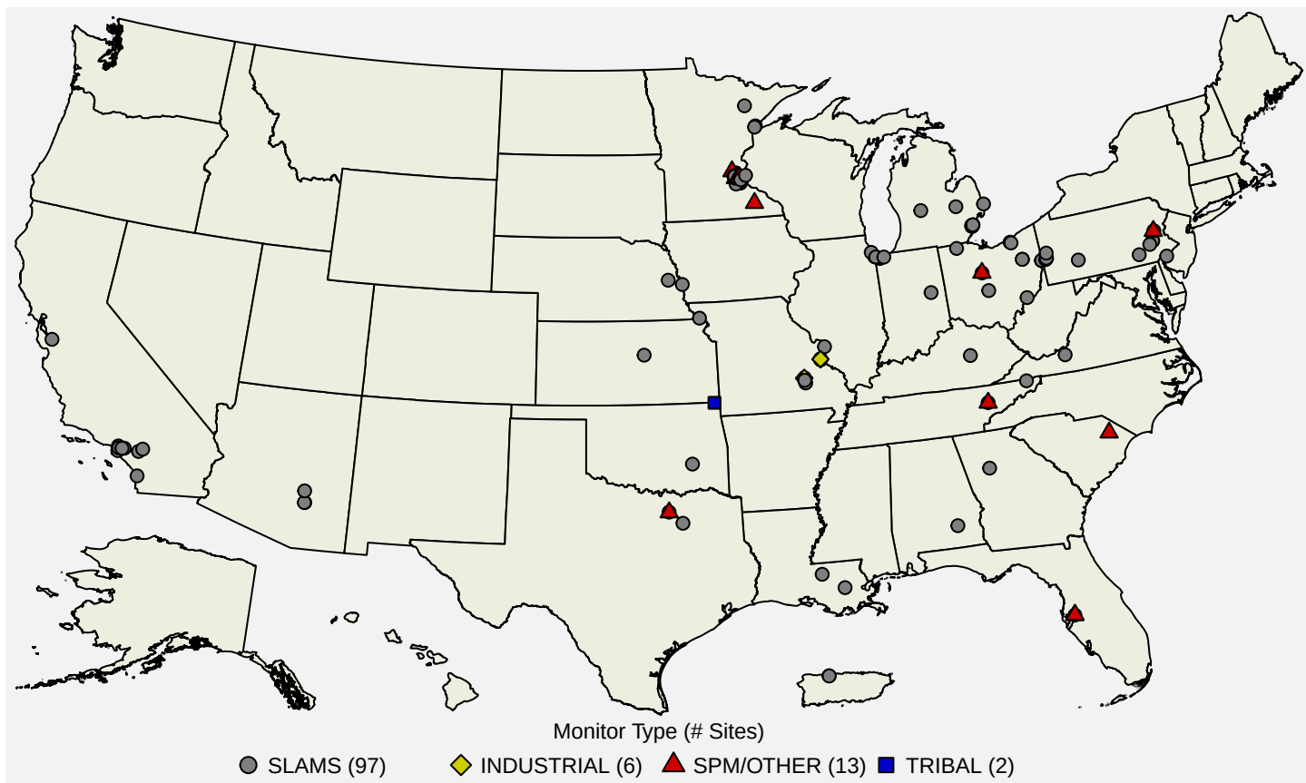
Figure 4: Map of U.S. ambient air monitoring sites reporting regulatory Pb data to the EPA during the 2023-2025 period. Source: AQS.
