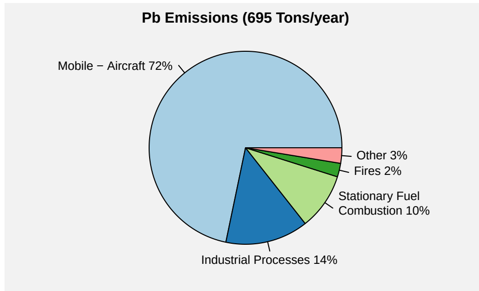
Figure 1. U.S. Pb emissions by sector. Source: 2023 NEI.
