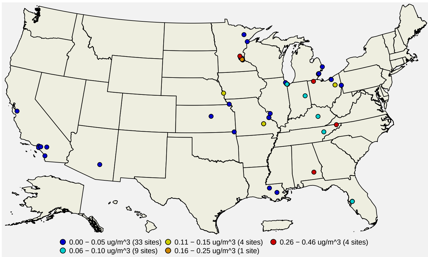
Figure 6: Pb design values in \mu\text{g}/\text{m}^3 for the 2023-2025 period. Source: AQS.
