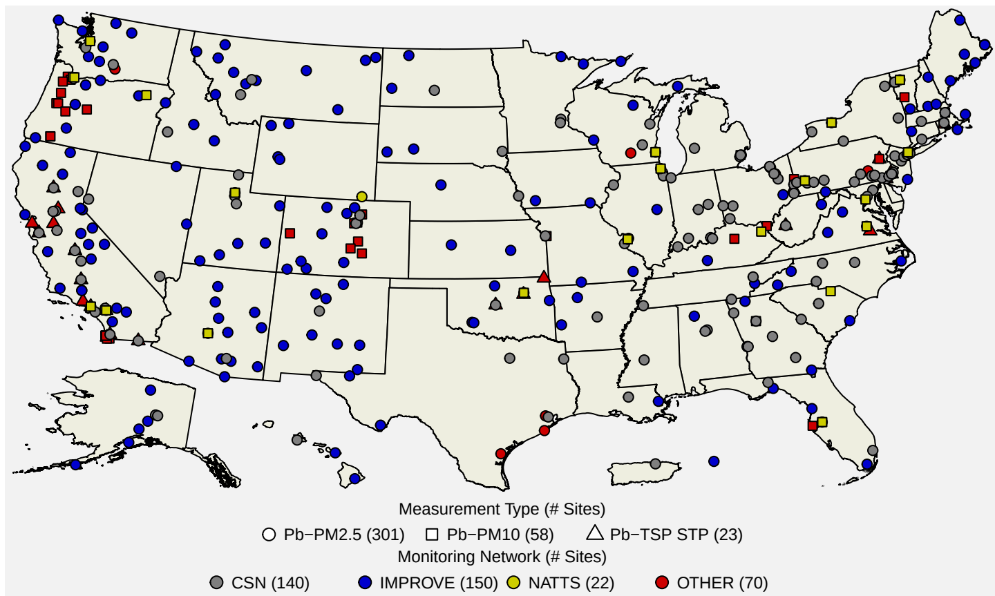
Figure 5: Map of U.S. ambient air monitoring sites reporting non-regulatory Pb data to the EPA during the 2023-2025 period. Source: AQS.
