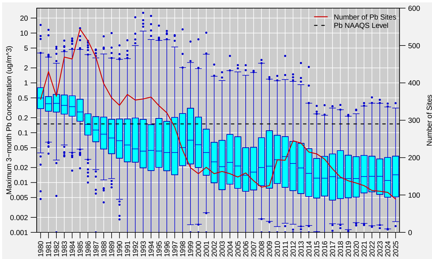
Figure 9: Distribution of annual maximum 3-month concentrations measured at regulatory Pb monitoring sites, 1980 to 2025. Boxes represent the median and interquartile range, whiskers extend to the 1st and 99th percentiles, and values outside this range are shown as circles. The red line shows the number of sites reporting regulatory data to EPA in each year. Note: the concentrations on the left-hand y-axis are shown on a logarithmic scale. Source: AQS.
