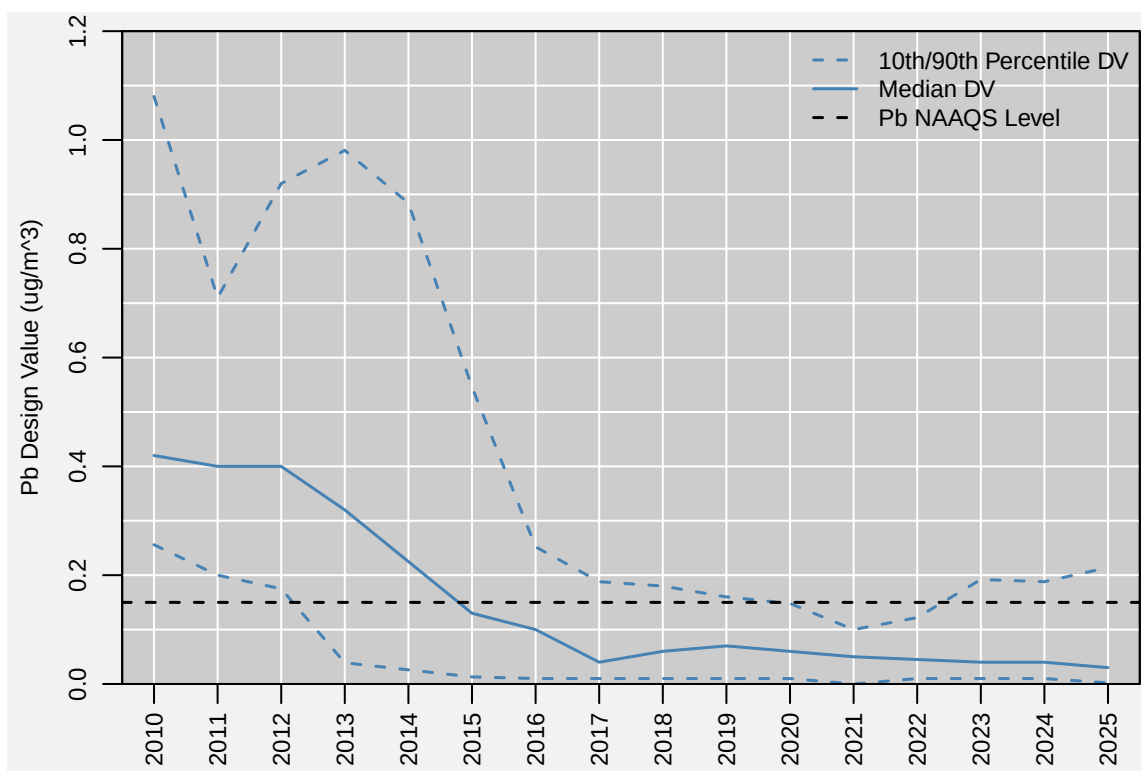
Figure 8: National trend in Pb design values in \mu\text{g}/\text{m}^3 , 2010 to 2025. Source: AQS.
