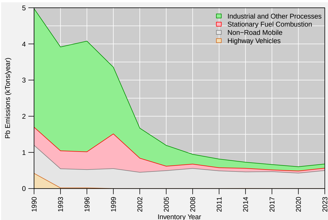
Figure 3. U.S. anthropogenic Pb emissions trend, 1990-2023. Source: Our Nation's Air: Status and Trends Through 2025
