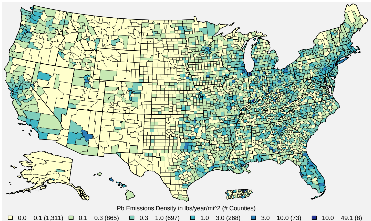
Figure 2. U.S. county-level Pb emissions density estimates in lbs/year/mi 2 . Source: 2023 NEI
