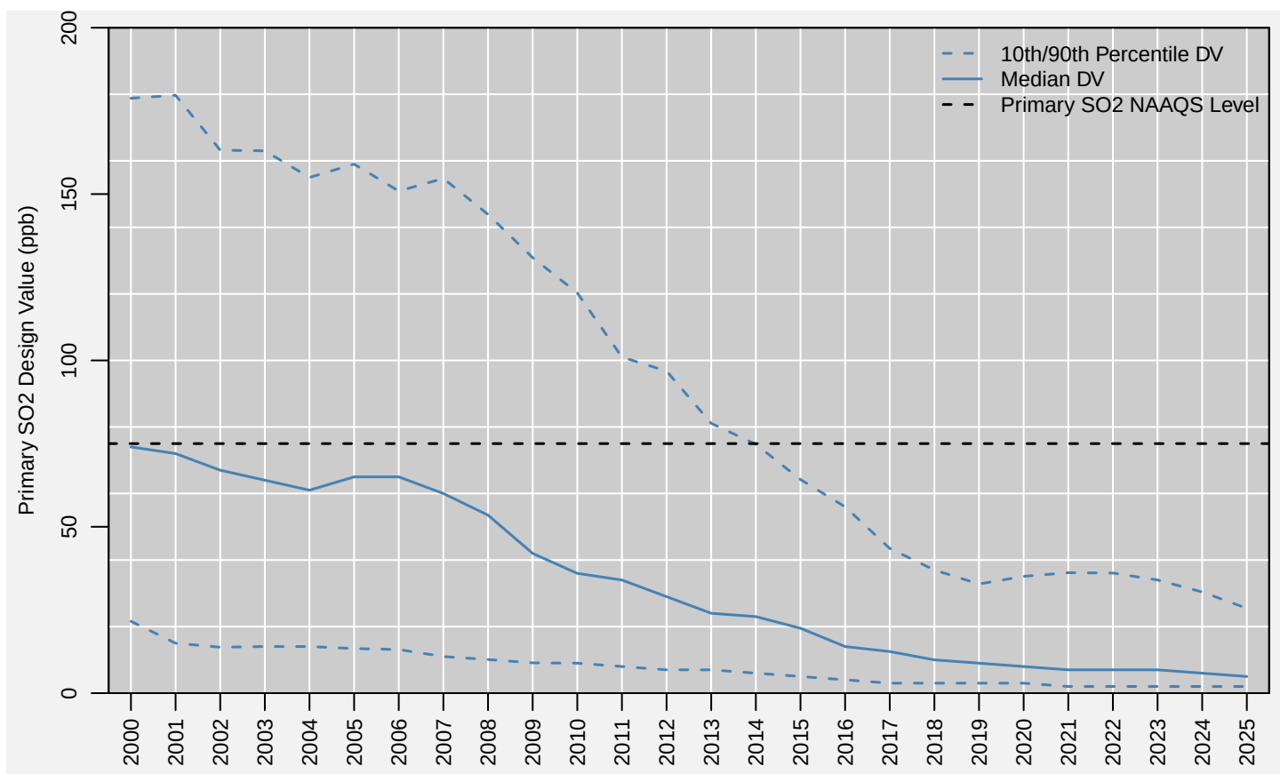
Figure 9: National trends in primary SO 2 design values in ppb, 2000 to 2025. Source: AQS.
