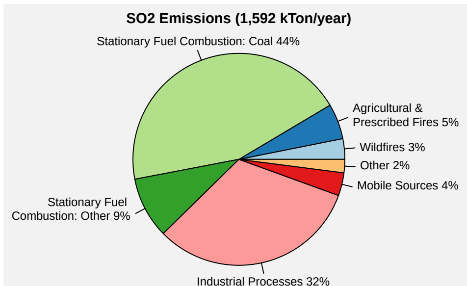
Figure 1. U.S. SO 2 emissions by sector. Source: 2023 NEI.
