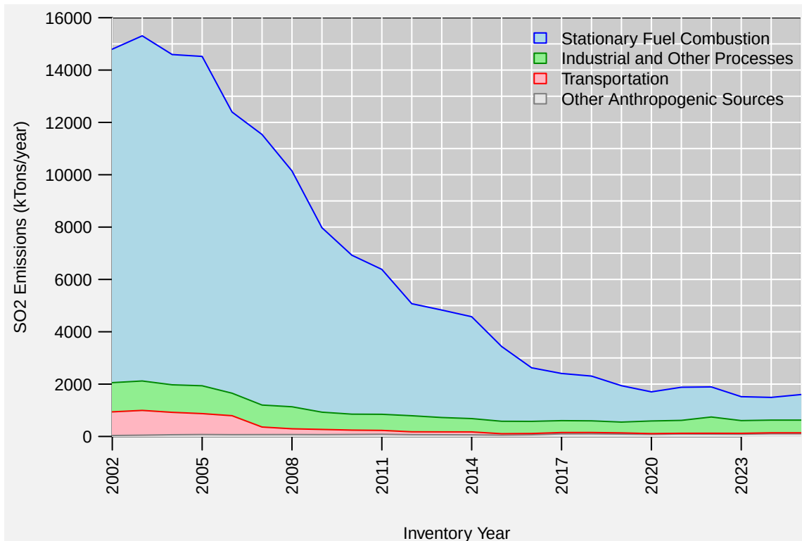
Figure 3. U.S. anthropogenic SO 2 emissions trend, 2002-2025. Source: EPA's Air Pollutant Emissions Trends Data
