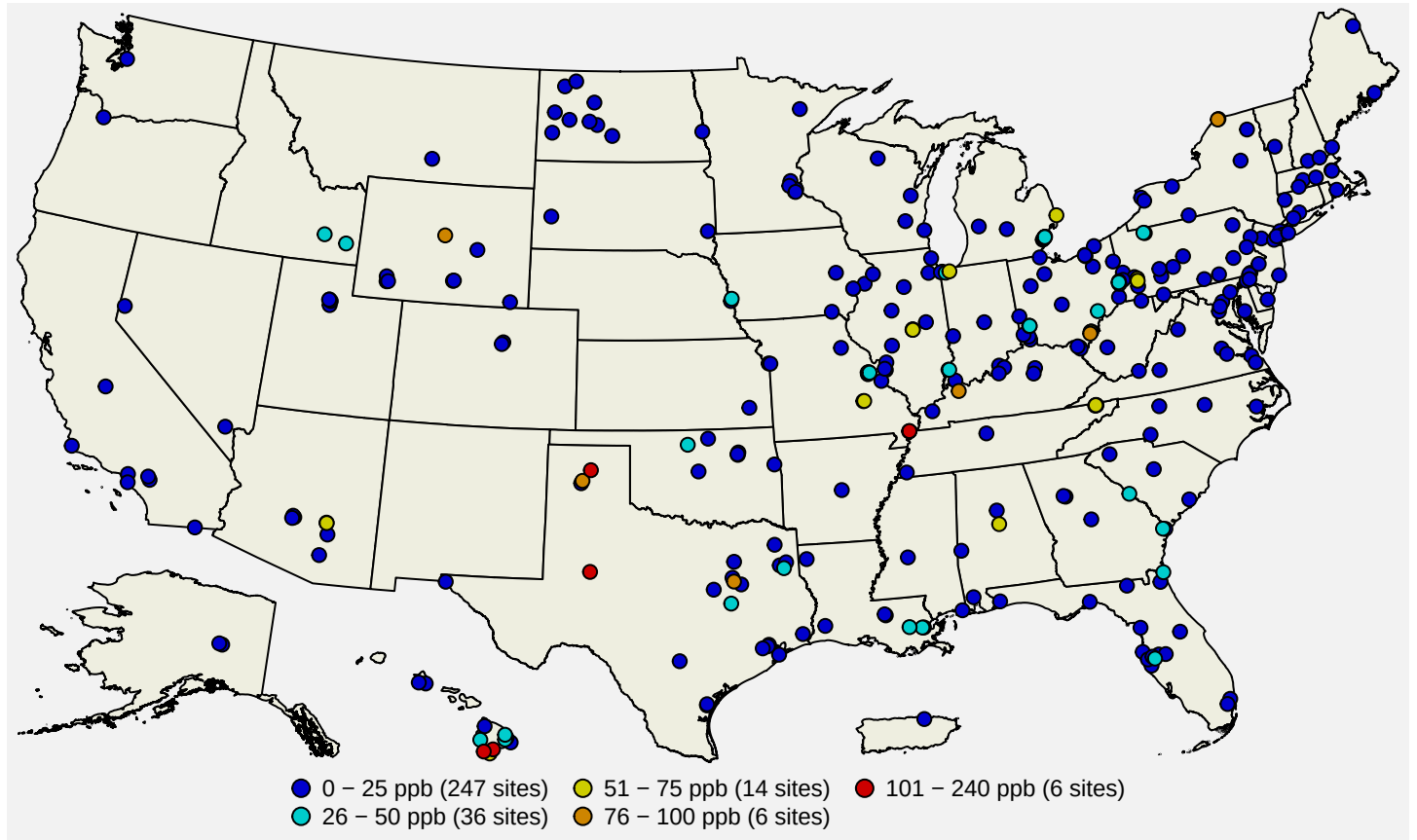
Figure 5: Primary SO 2 design values in ppb for the 2023-2025 period. Source: AQS.
