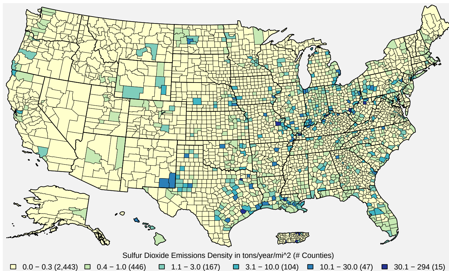
Figure 2. U.S. county-level SO 2 emissions density estimates in tons/year/mi 2 . Source: 2023 NEI
