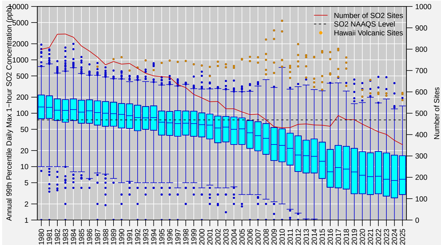
Figure 11: Distribution of annual 99th percentile MDA1 SO 2 concentrations measured at U.S. monitoring sites, 1980 to 2025. Boxes represent the median and interquartile range, whiskers extend to the 1st and 99th percentiles, and values outside this range are shown as circles. 5 The red line shows the number of SO 2 monitoring sites reporting data to EPA in each year. Source: AQS.
