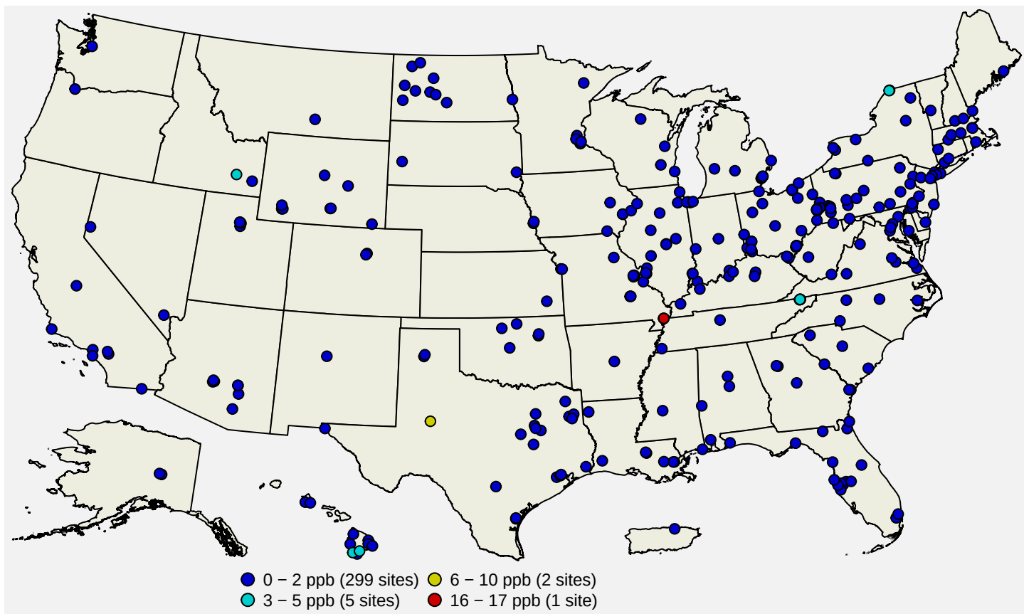
Figure 6: Secondary SO 2 design values in ppb for the 2023-2025 period. Source: AQS.
