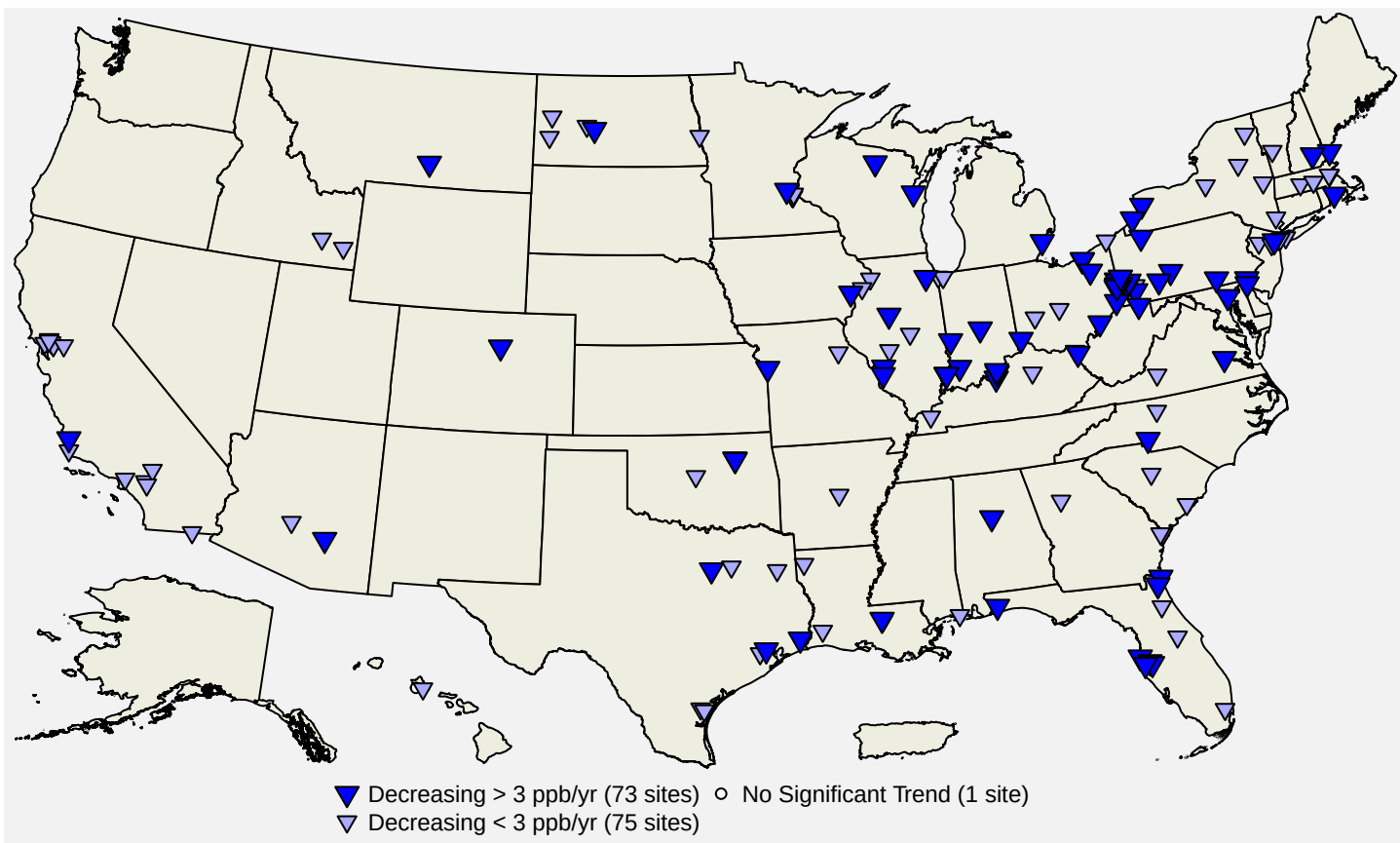
Figure 7: Site-level trends in primary SO 2 design values based on data from 2000 through 2025. Source: AQS, trends computed using R statistical software.
