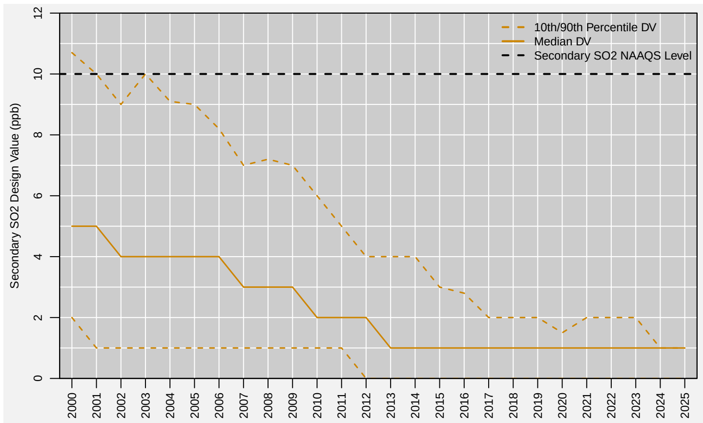
Figure 10: National trends in secondary SO 2 design values in ppb, 2000 to 2025. Source: AQS.
