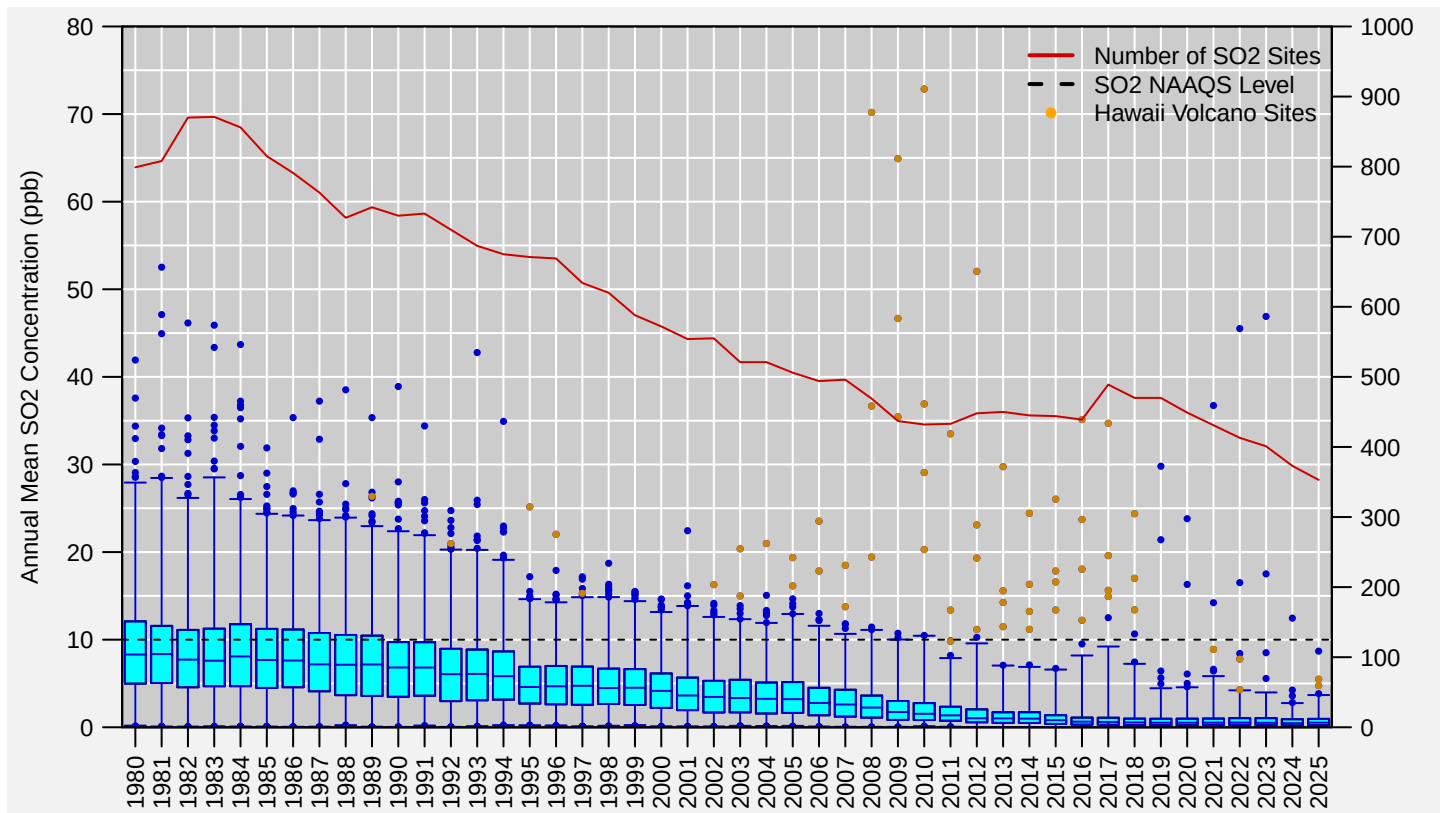
Figure 12: Distribution of annual mean SO 2 concentrations measured at U.S. monitoring sites, 1980 to 2025. Boxes represent the median and interquartile range, whiskers extend to the 1st and 99th percentiles, and values outside this range
