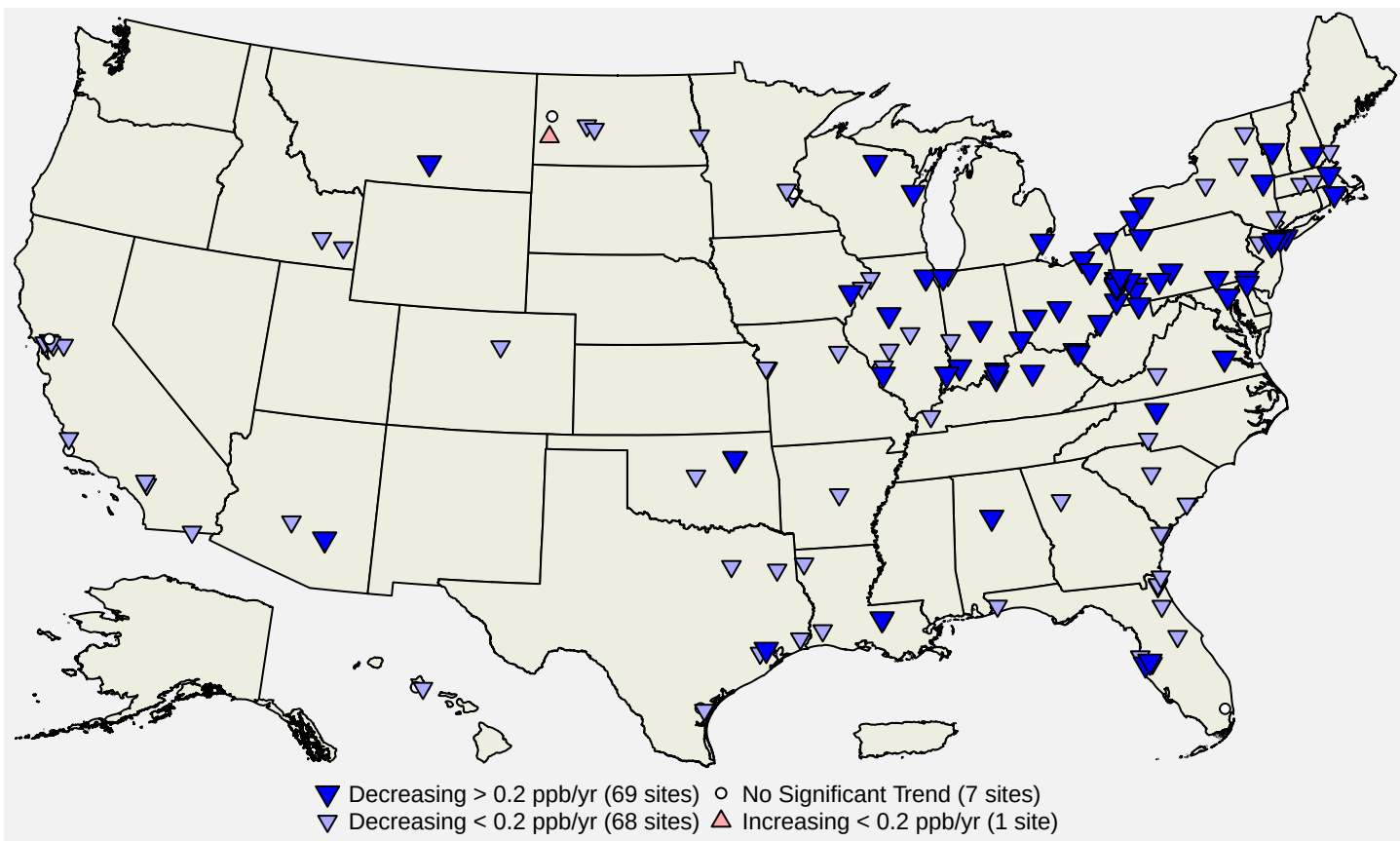
Figure 8: Site-level trends in secondary SO 2 design values based on data from 2000 through 2025. Source: AQS, trends computed using R statistical software.
