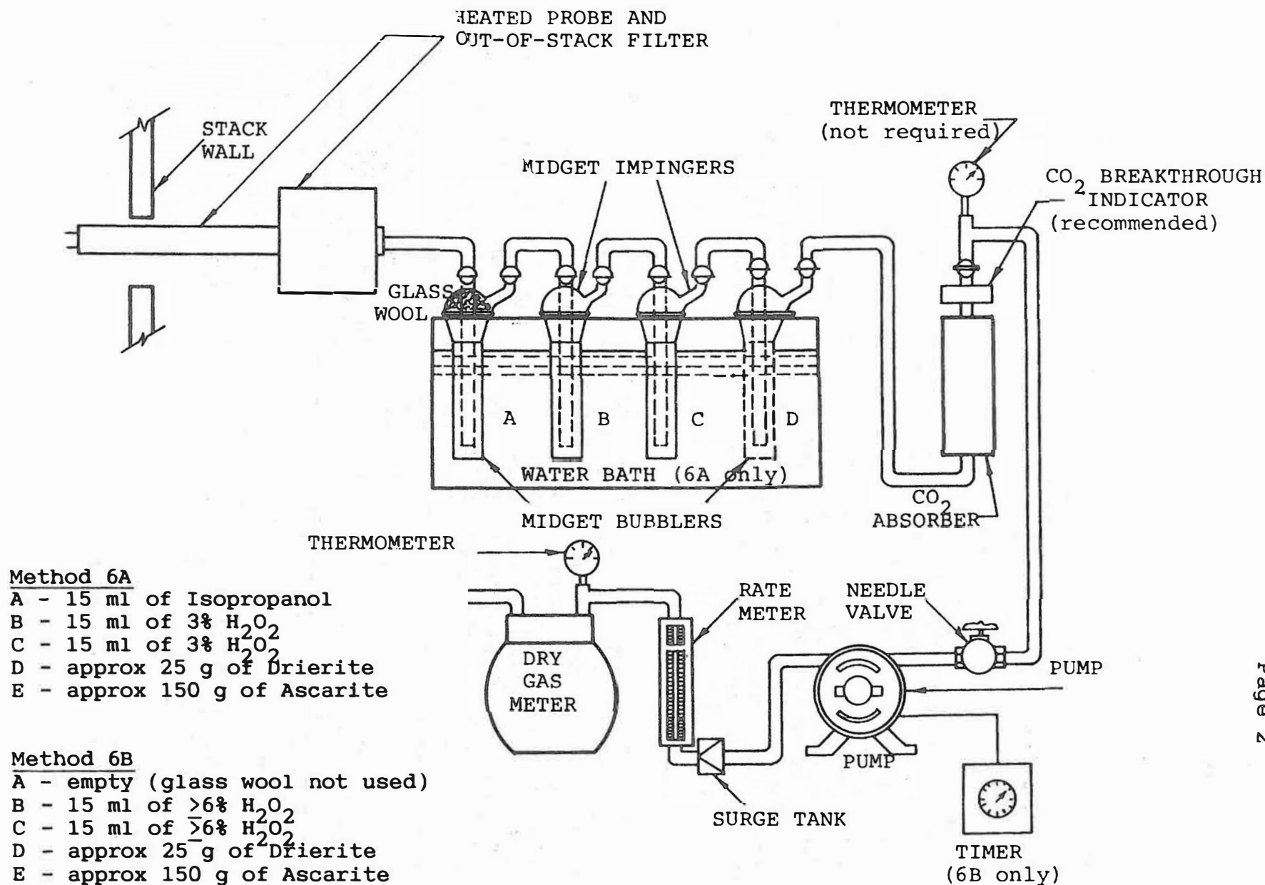
Figure 1.1. Sampling train.
