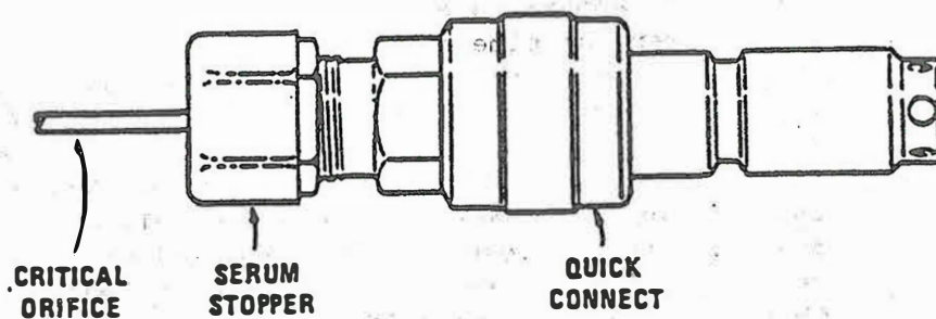
Critical orifice adaptation to Method 5-type metering system.
