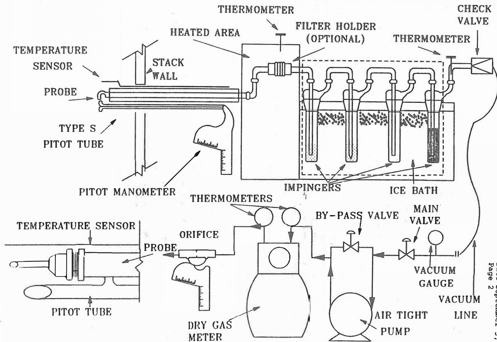
Figure 1.1. Schematic of Method 101A sampling train.
