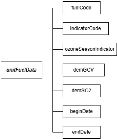
Figure 9: unitFuelData JSON Elements
