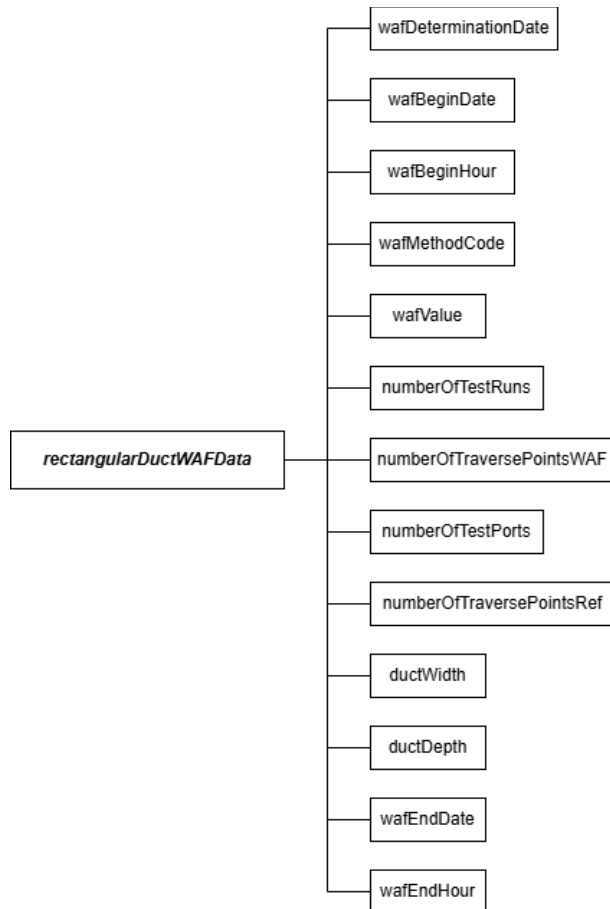
Figure 15: rectangularDuctWAFData JSON Elements
