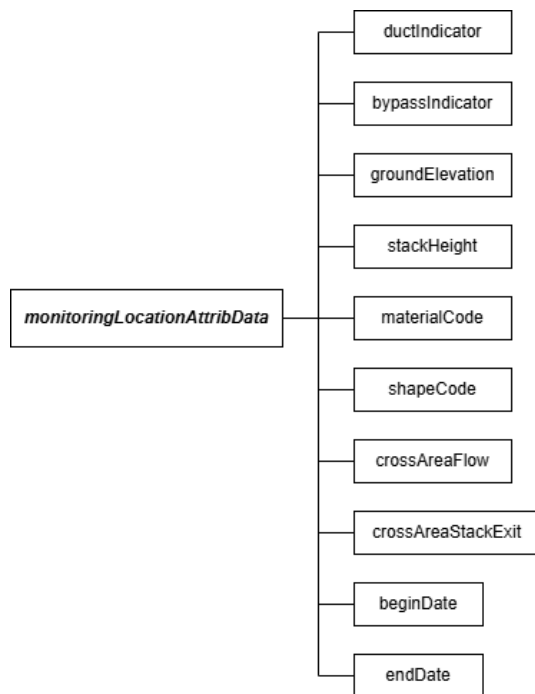
Figure 6: monitoringLocationAttribData JSON Elements
