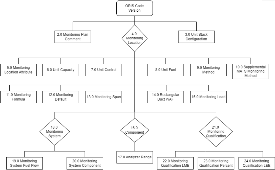
Figure 1: Monitoring Plan Data JSON Schema
