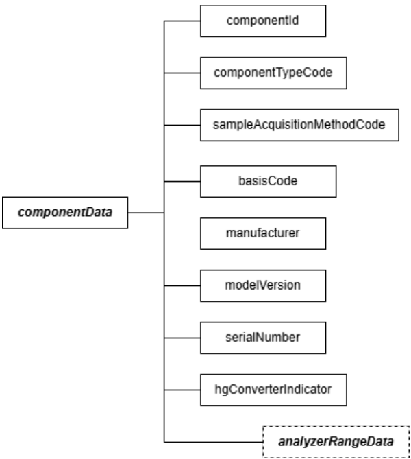
Figure 17: componentData JSON Elements
