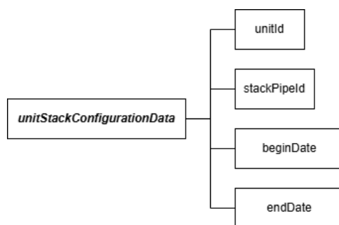
Figure 4: unitStackConfigurationData JSON Elements
