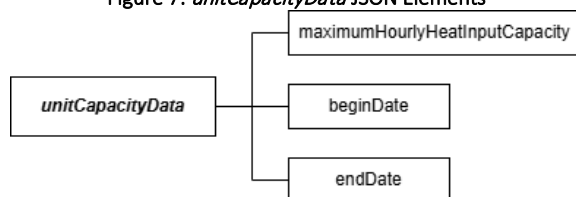
Figure 7: unitCapacityData JSON Elements
