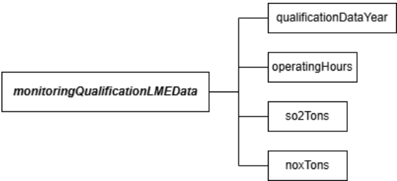
Figure 23: monitoringQualificationLMEData JSON Elements
