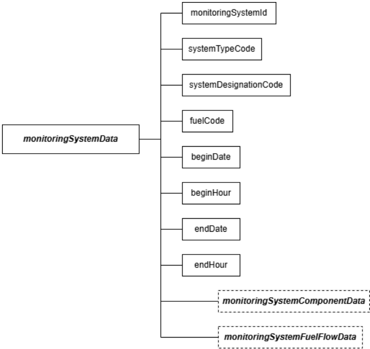
Figure 19: monitoringSystemData JSON Elements
