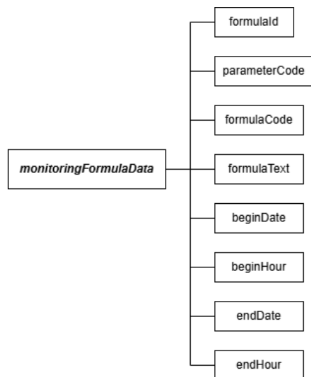
Figure 12: monitoringFormulaData JSON Elements
