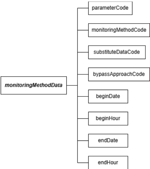
Figure 10: monitoringMethodData JSON Elements
