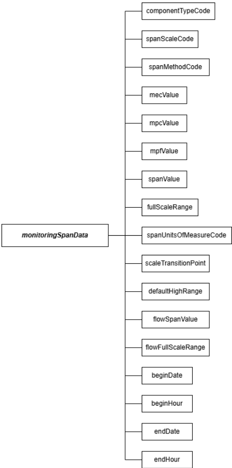
Figure 14: monitoringSpanData JSON Elements
