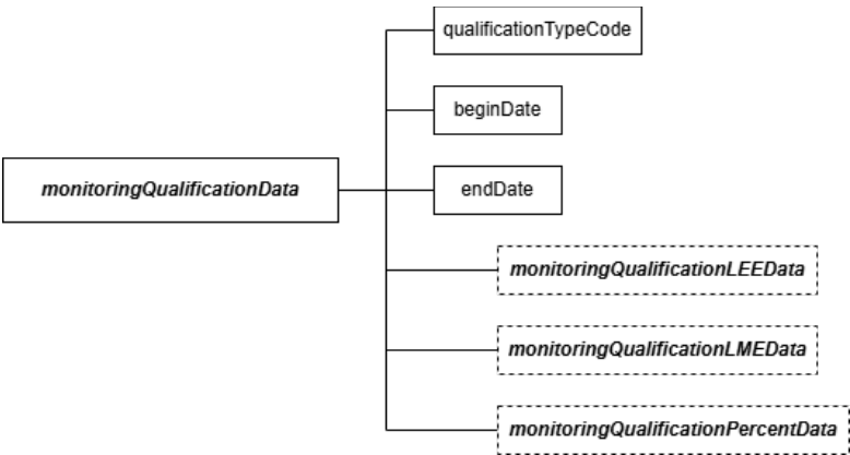
Figure 22: monitoringQualificationData JSON Elements
