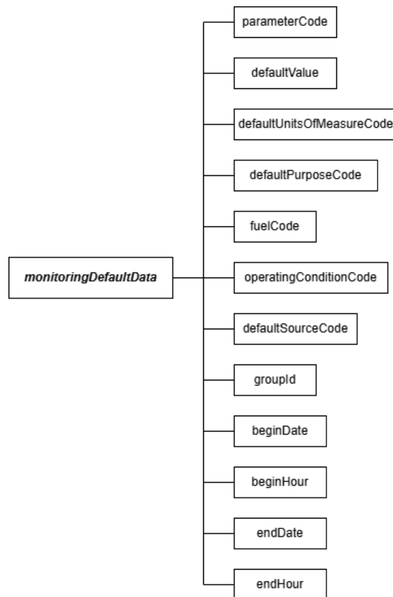
Figure 13: monitoringDefaultData JSON Elements
