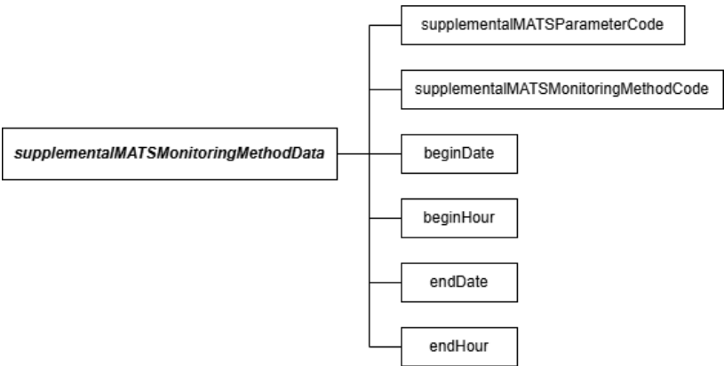
Figure 11: supplementalMATSMonitoringMethodData JSON Elements
