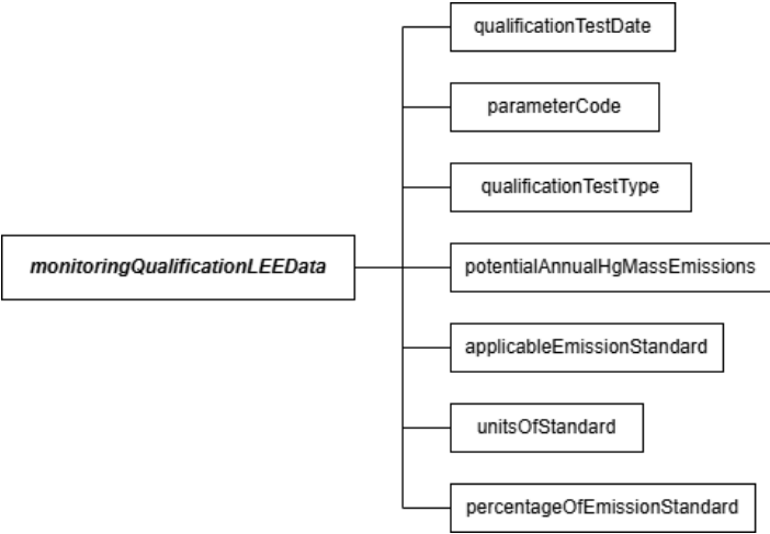
Figure 25: monitoringQualificationLEEData JSON Elements
