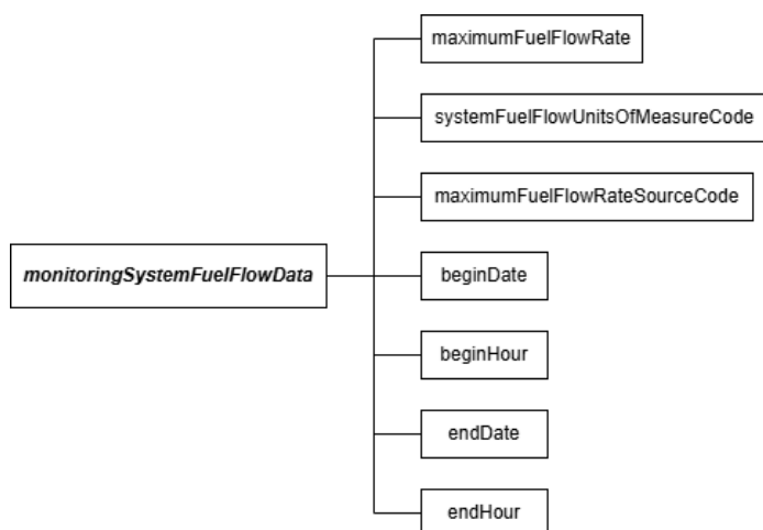
Figure 20: monitoringSystemFuelFlowData JSON Elements
