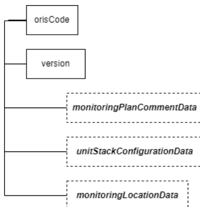
Figure 2: Monitoring Plan JSON Elements
