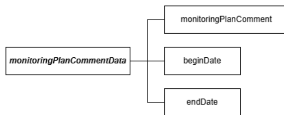
Figure 3: monitoringPlanCommentData JSON Elements
