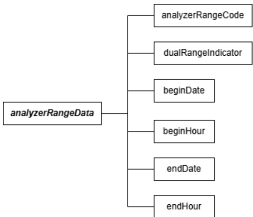
Figure 18: analyzerRangeData JSON Elements
