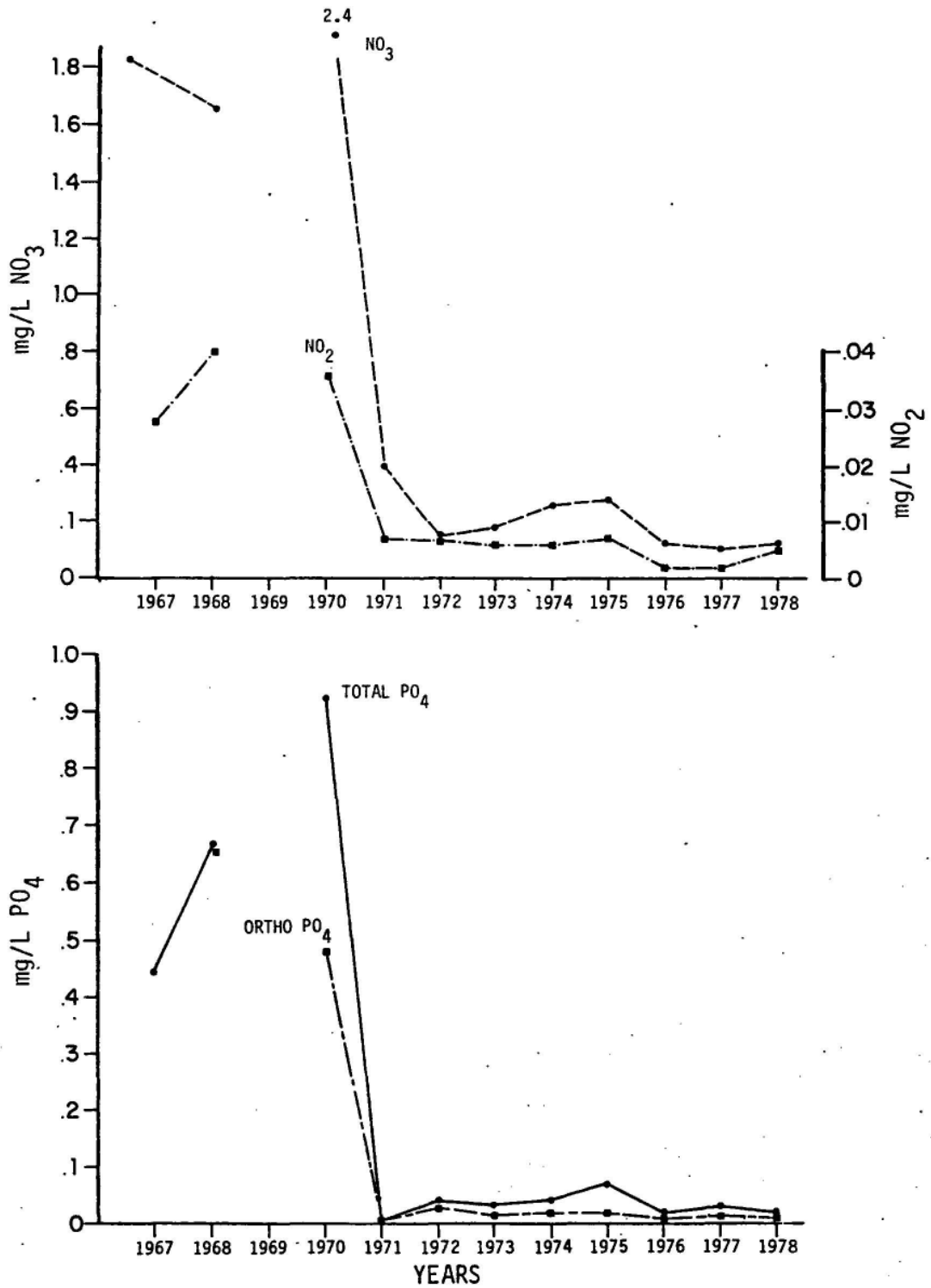
Figure 5-1. Seasonal Mean Nutrient Concentrations in Hooksett Pond - 1967-1978 (Merrimack River Summary Report, Normandeau 1979)
