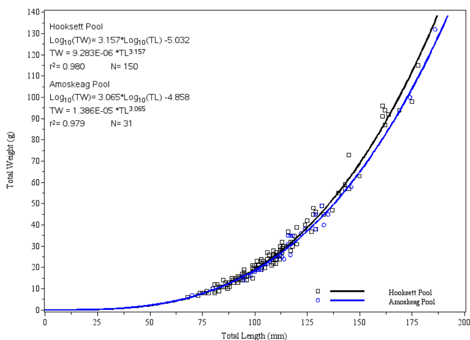
Figure 4-10-2. Empirical length-weight relations for redbreast sunfish captured via electrofishing within Hooksett and Amoskeag Pools during 2011.
