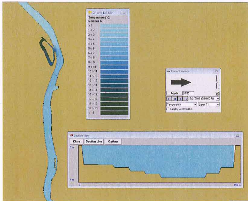
Figure 3-12. Model predicted delta temperature contours at 50 th percentile upstream ambient condition during summer biological period for an extreme year: 13-20 August 2001. Surface temperatures and cross section at S4 shown.
