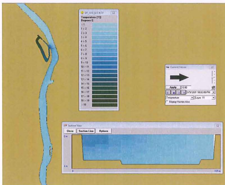
Figure 3-11. Model predicted delta temperature contours at 50 th percentile upstream ambient condition during summer period for an extreme year: 13-20 August 2001. Surface temperatures and cross section at S0 shown.
