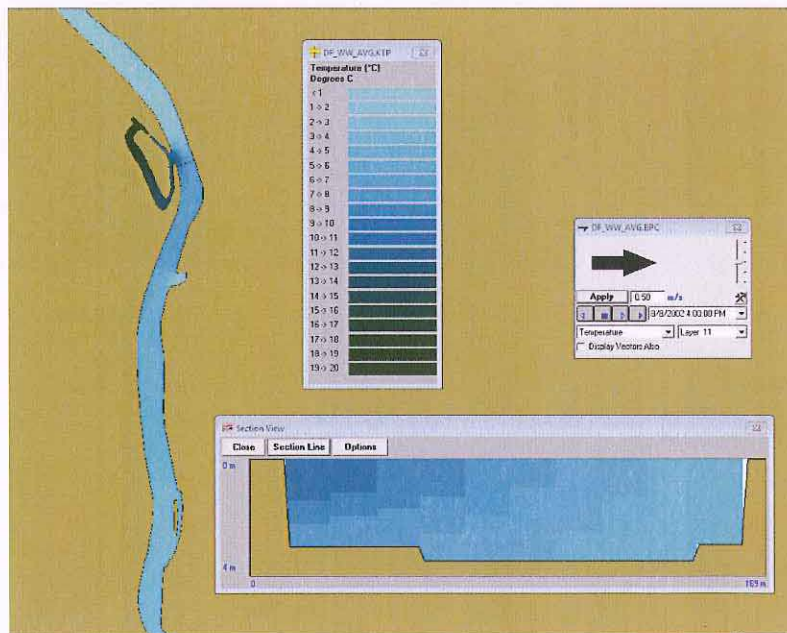
Figure 3-9. Model predicted delta temperature contours at 50 th percentile upstream ambient condition during summer biological period for an average year: 13-20 August 2002. Surface temperatures and cross section at S0 shown.
