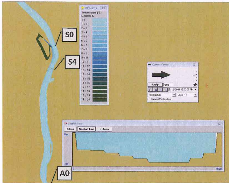
Figure 3-2. Model predicted delta temperature contours at 50 th percentile upstream ambient condition during the early spring biological period for an average year: 7-14 May 2004. Surface temperatures and cross section at S4 shown.
