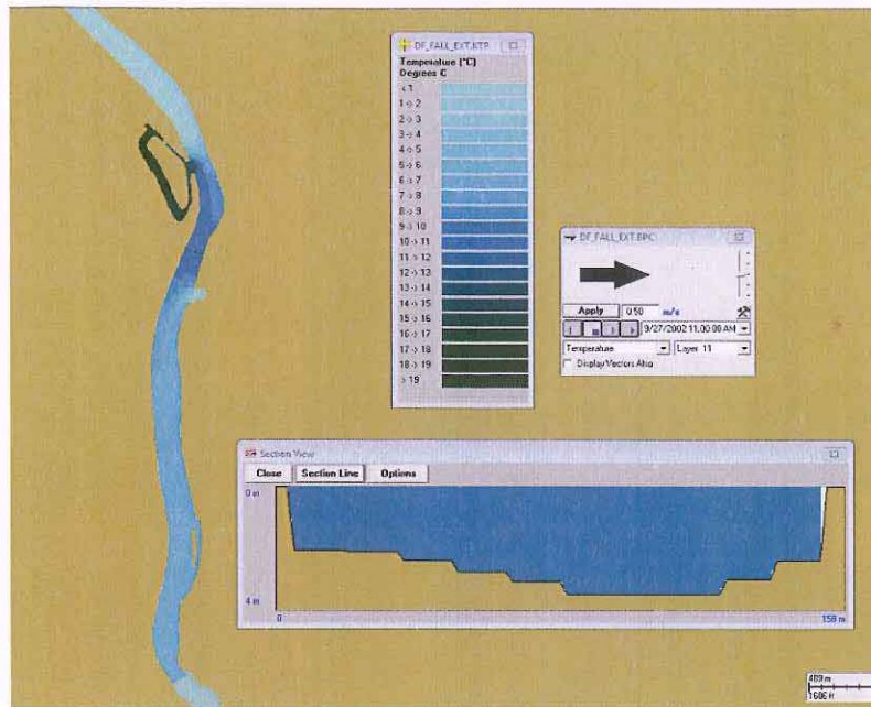
Figure 3-16. Model predicted delta temperature contours at 50 th percentile upstream ambient condition during fall biological period for an extreme year: 24-30 September 2002. Surface temperatures and cross section at S4 shown.
