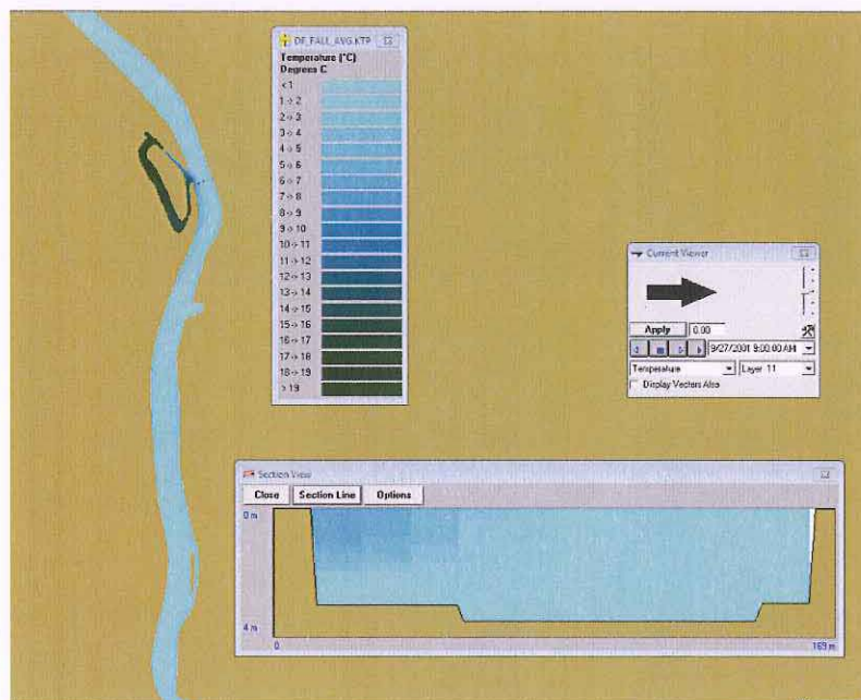
Figure 3-13. Model predicted delta temperature contours at 50 th percentile upstream ambient condition during fall biological period for an average year: 24-30 September 2001. Surface temperatures and cross section at S0 shown.
