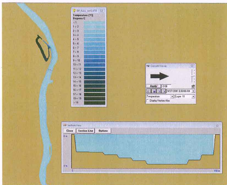
Figure 3-14. Model predicted delta temperature contours at 50 th percentile upstream ambient condition during fall biological period for an average year: 24-30 September 2001. Surface temperatures and cross section at S4 shown.
