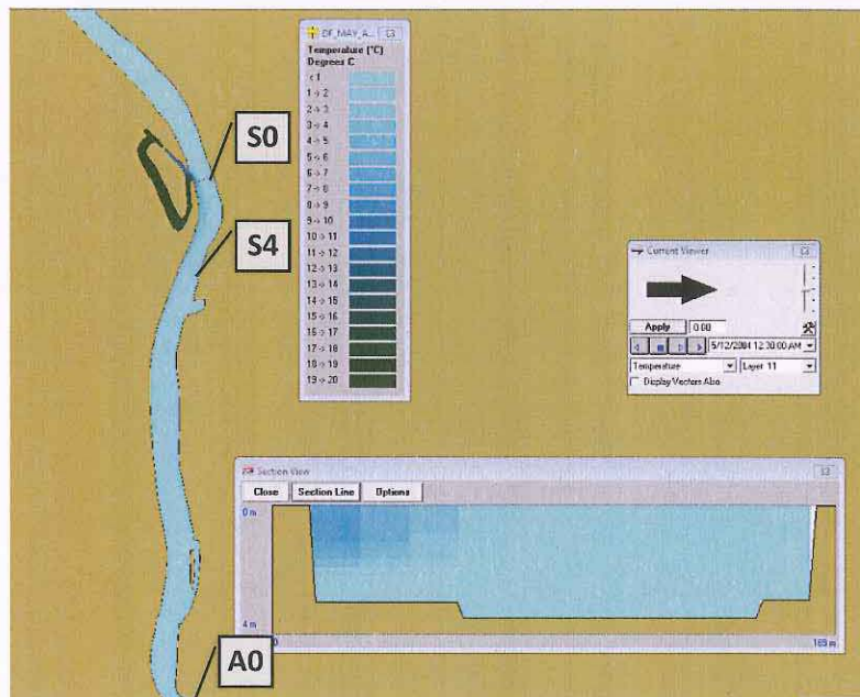
Figure 3-1. Model predicted delta temperature contours at 50 th percentile upstream ambient condition during the early spring biological period for an average year: 7-14 May 2004. Surface temperatures and cross section at S0 shown.
