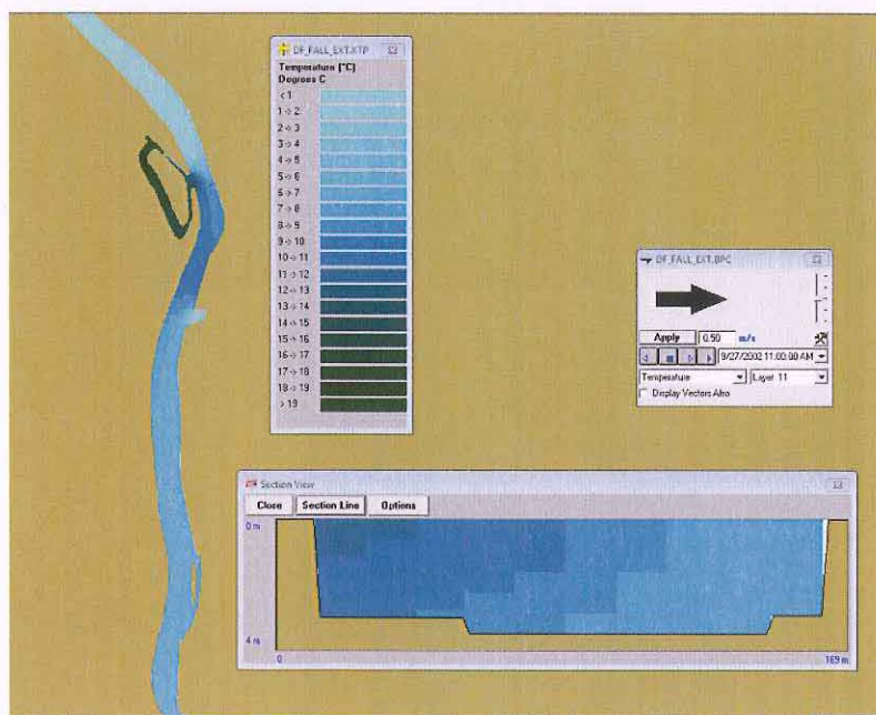
Figure 3-15. Model predicted delta temperature contours at 50 th percentile upstream ambient condition during fall biological period for an extreme year: 24-30 September 2002. Surface temperatures and cross section at S0 shown.
