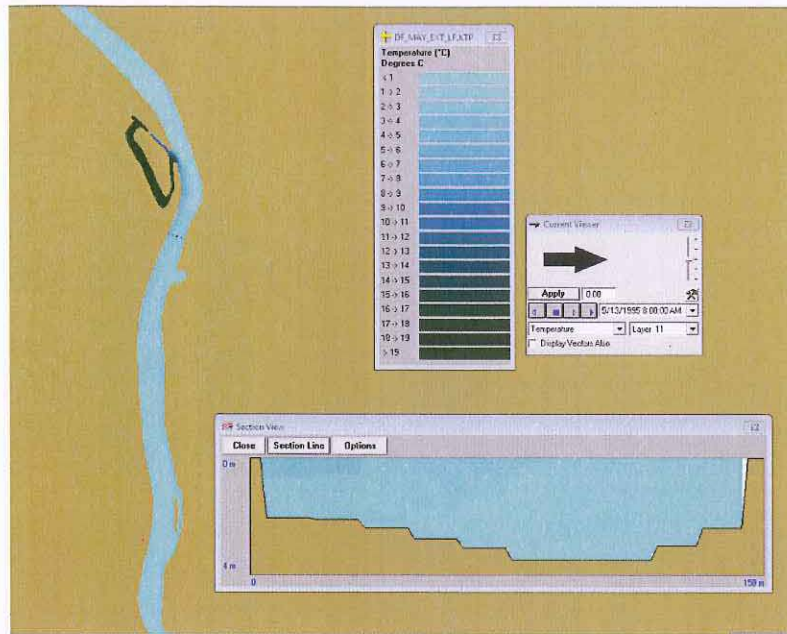
Figure 3-4. Model predicted delta temperature contours at 50 th percentile upstream ambient condition during the early spring biological period for an extreme year: 7-14 May 1995. Surface temperatures and cross section at S4 shown.
