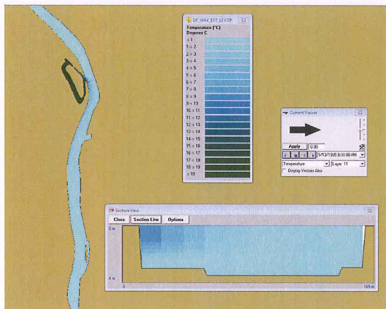
Figure 3-3. Model predicted delta temperature contours at 50 th percentile upstream ambient condition during the early spring biological period for an extreme year: 7-14 May 1995. Surface temperatures and cross section at S0 shown.
