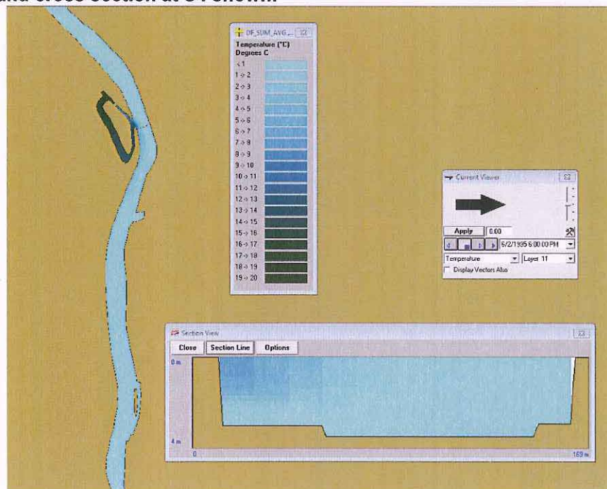
Figure 3-5. Model predicted delta temperature contours at 50 th percentile upstream ambient condition during the late spring biological period for an average year: 7-14 June 1995. Surface temperatures and cross section at S0 shown.
