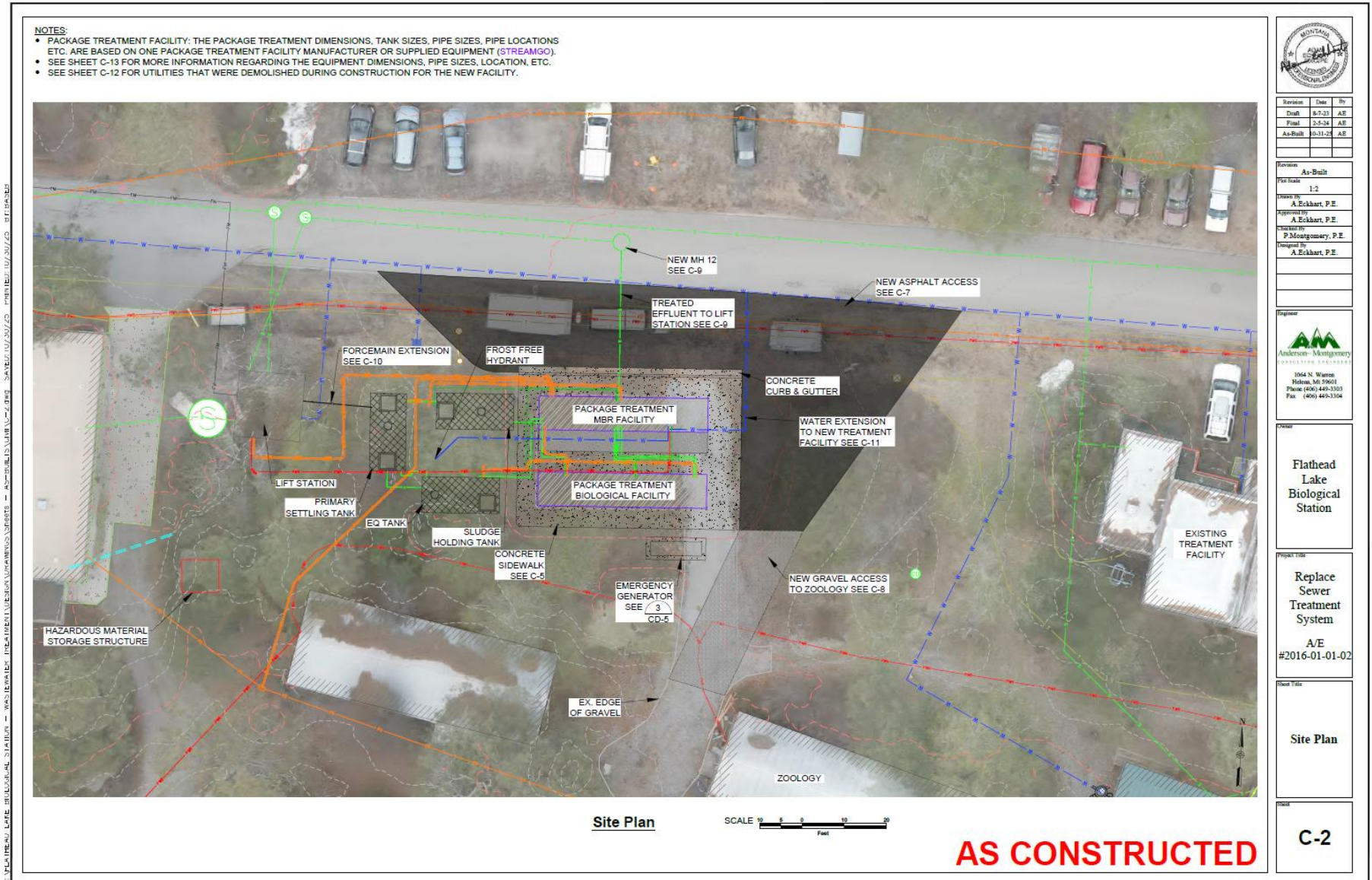
Figure 3. Site Plan
