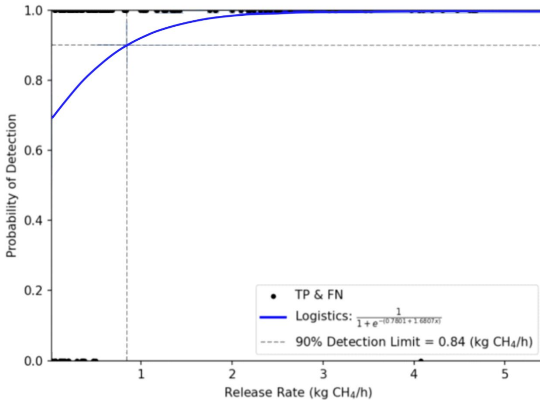
Figure 7: SENSIA RedLook System MATM utilizing the Caroline FY OGI camera non-wind normalized PoD curve. PoD versus emission rate (kg CH 4 /hr) assessed with logistic regression including all true positives and false negatives. True positives and false negative detections are shown with markers at y=1 and y=0, respectively. The regression is performed on bootstrapped results to show a cloud of curves to illustrate uncertainty in the result.
