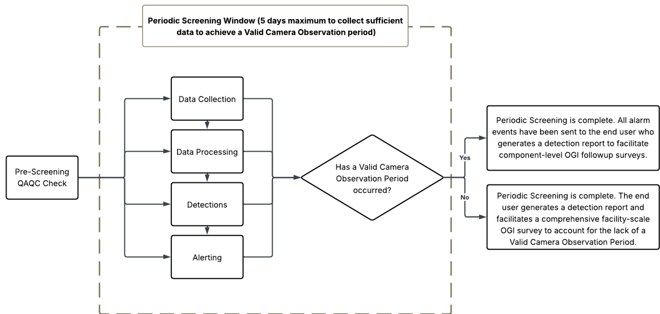
Figure 5. SENSIA RedLook System MATM periodic screening workflow.
