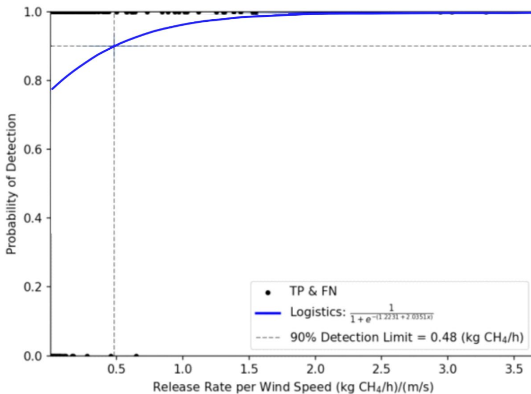
Figure 8: SENSIA RedLook System MATM utilizing the Caroline FY OGI camera wind normalized PoD curve. PoD versus wind normalized emission rate (kg CH 4 /hr)/(m/s) assessed with logistics regression. including all true positives and false negatives. True positive and false negative detections are shown with markers at y=1 and y=0, respectively.
