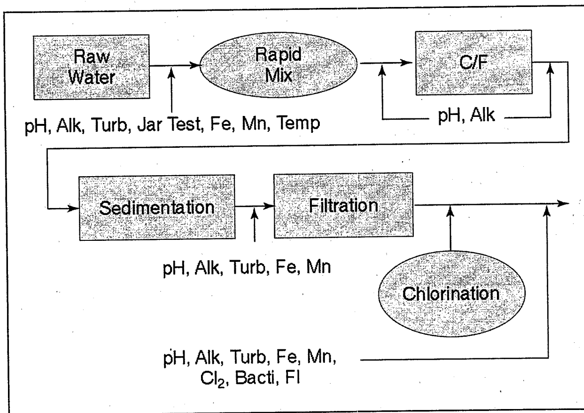
Figure 3-22. Typical Water Quality Monitoring Plan Layout for a Surface Water Treatment Facility
