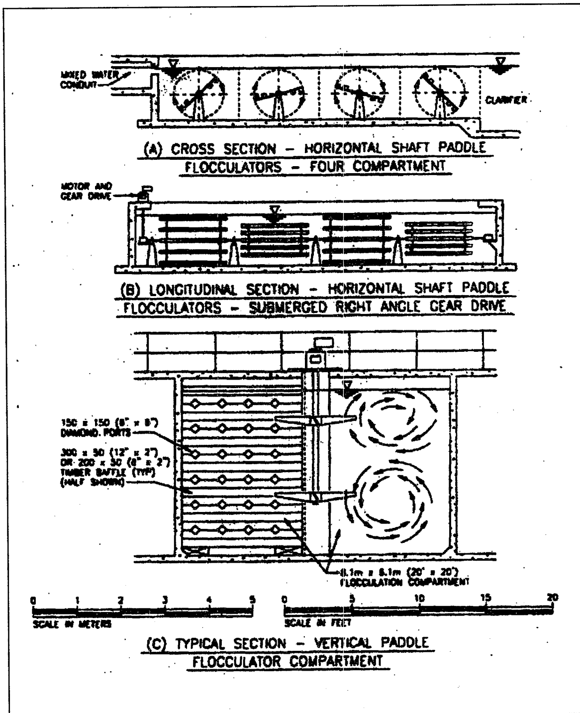
Figure 3-11. Mechanical Flocculator Types
