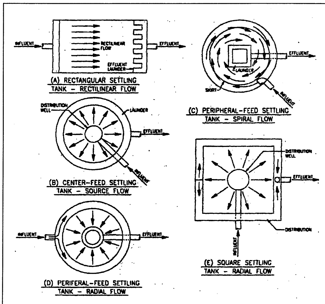
Figure 3-12. Different Clarifier Shapes
