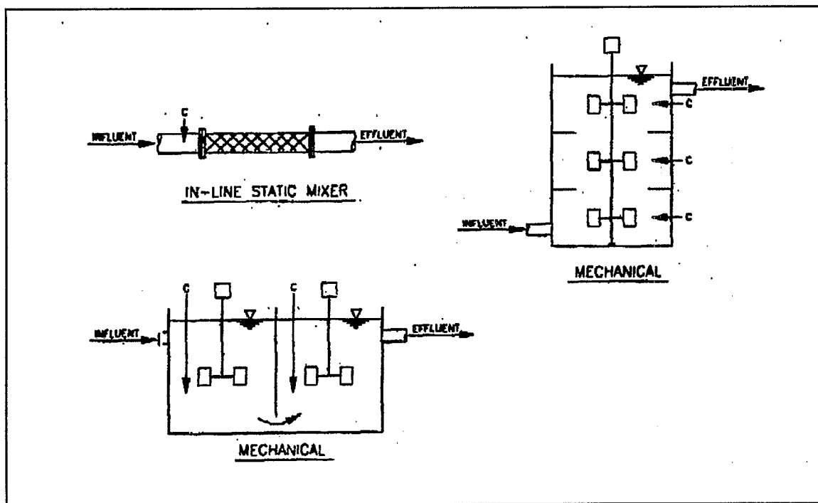
Figure 3-7. Schematic Drawings of Types of Rapid Mix Unit Configurations
