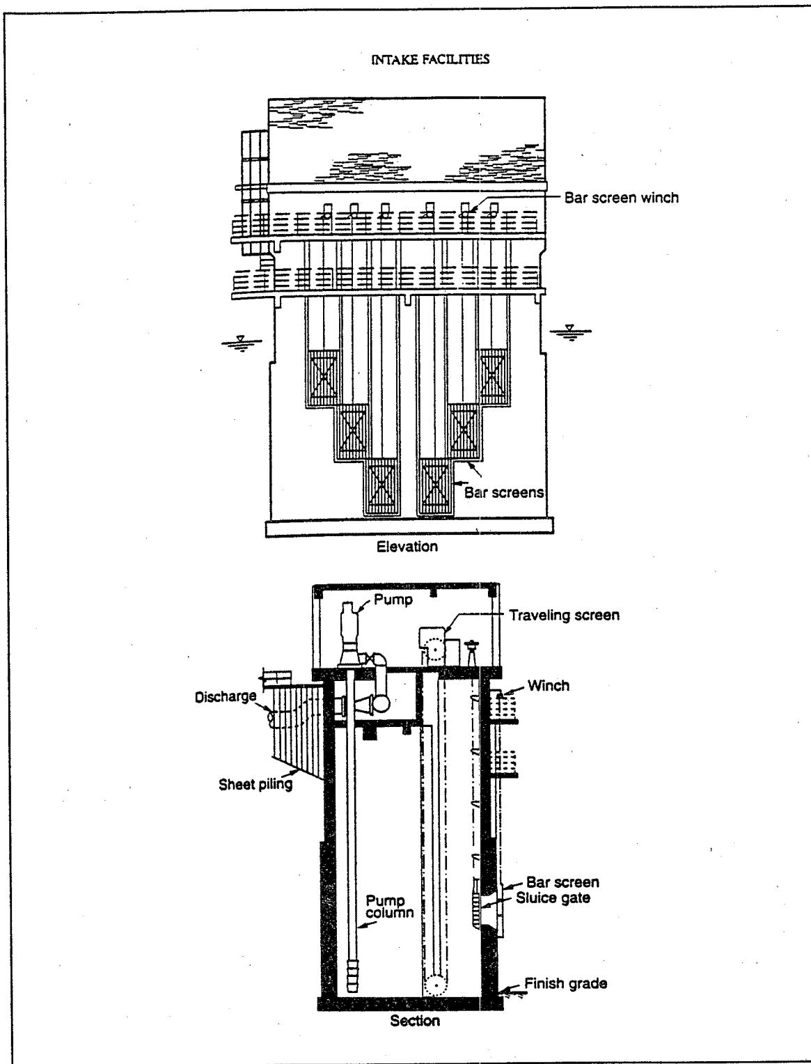
Figure 3-2. Surface Water Intake with Multiple Level Withdrawals
