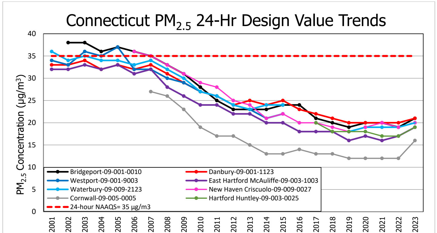
Figure 2-4. Long-term trends in PM 2.5 24-hour design values at each of Connecticut's monitors shown in relation to the standard.
