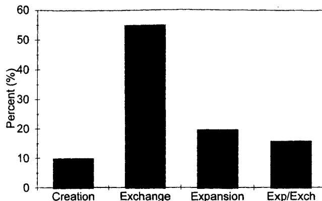
Figure 5. Distribution of mitigation wetlands (MWs) ( n = 51 ) by method of construction (mitigation method). Mitigation methods used for wetlands included in this study are creation, exchange, expansion, and a combination of exchange and expansion (Exp/Exch) and are described in Table 1.
