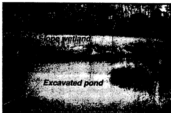
Figure 3. Diagrams and photographs of wetlands representative of the regional atypical HGM classes: A) depression-in-riverine setting, B) in-stream-depression, and C) depression-in-slope-setting.
