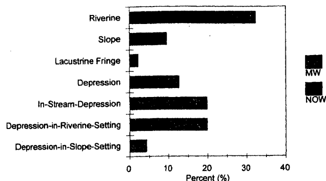
Figure 4. Landscape profile for naturally occurring wetlands (NOWs) ( n = 45 ) and mitigation wetlands (MWs) ( n = 51 ) in the Portland, Oregon metropolitan area (the All Site-Profile). Wetlands are distributed among the four regional hydrogeomorphic (HGM) types (riverine, slope, lacustrine fringe, and depression) and the three regional atypical HGM types (in-stream-depression, depression-in-riverine-setting, and depression-in-slope-setting).
