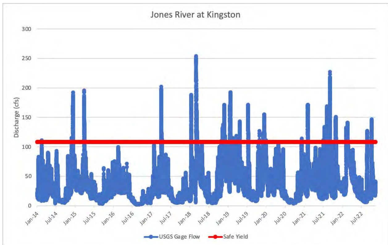
Figure 7. Streamflow for the Jones River at Kingston (USGS Gage 01105870) depicted in blue. Safe Yield is for the South Coastal Basin which includes the Jones River watershed, shown in red. Time period extends from January 2014 through November 2022. Source: Mass Rivers Alliance.
