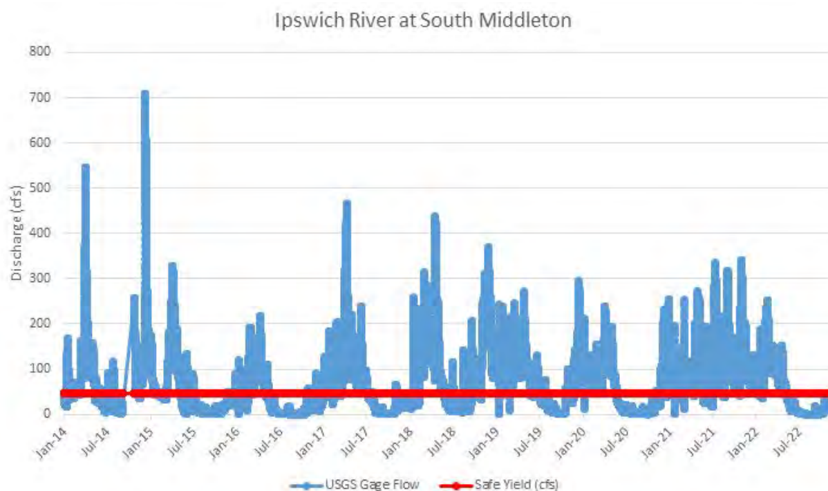
Figure 5. Streamflow for Ipswich River at South Middleton (USGS Gage 01101500) depicted in blue. Safe Yield for the Ipswich River Basin shown in red. Time period from January 2014 to November 2022. Source: Mass Rivers Alliance.
