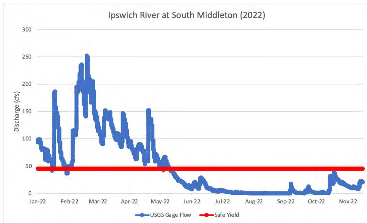
Figure 2. Streamflow for Ipswich River at South Middleton (USGS Gage 01101500) depicted in blue. Safe Yield for the Ipswich River Basin shown in red. Time period from January 2022 to November 2022. Source: Mass Rivers Alliance.
