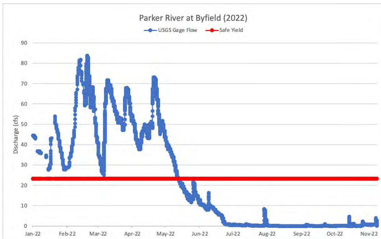
Figure 1. Streamflow for the Parker River at Byfield (USGS Gage 01101000) depicted in blue. Safe Yield for the Parker River Basin shown in red. Time period from January 2022 to November 2022. Source: Mass Rivers Alliance.
