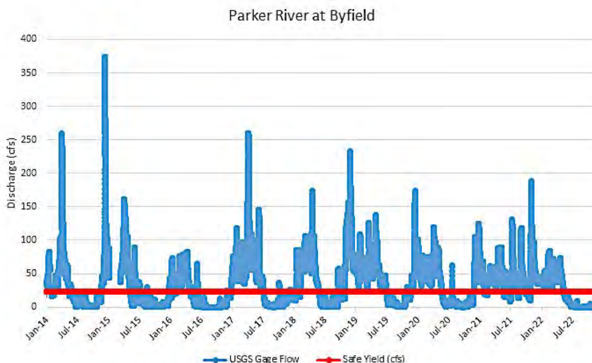
Figure 4. Streamflow for the Parker River at Byfield (USGS Gage 01101000) depicted in blue. Safe Yield for the Parker River Basin shown in red. Time period extends from January 2014 to November 2022. Source: Mass Rivers Alliance.
