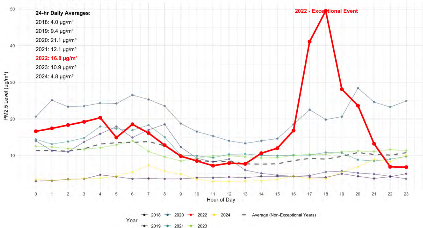
Hourly PM2.5 Levels on April 4th Across Years Forrest County - Exceptional Event Highlighted (2022)
