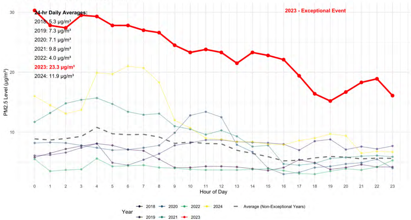
Hourly PM2.5 Levels on August 27th Across Years Forrest County - Exceptional Event Highlighted (2023)
