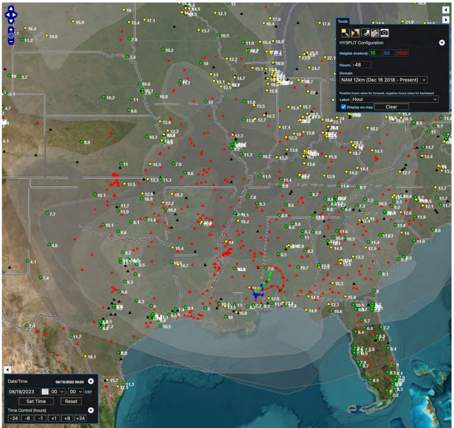
The AirNowTech Navigator image from August 19 th , 2023, shows a batch of smoke from Canadian wildfires that was transported down encompasses all the Mid-South and southeastern United States. Overlaid are 48-hour back trajectories, showing very little movement at 10m, 50m, and 1500m, indicating very stagnant conditions.
