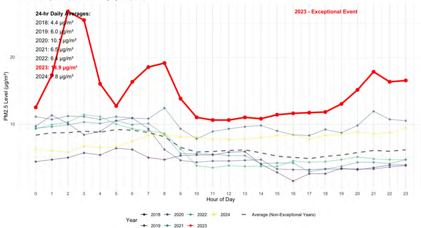
Hourly PM2.5 Levels on August 18th Across Years Forrest County - Exceptional Event Highlighted (2023)
