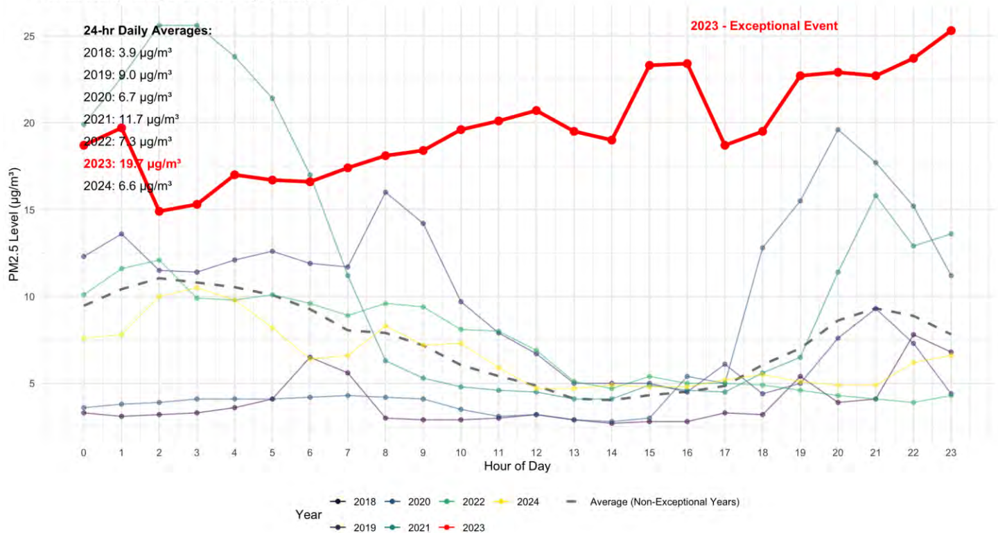
Hourly PM2.5 Levels on March 7th Across Years Forrest County - Exceptional Event Highlighted (2023)
