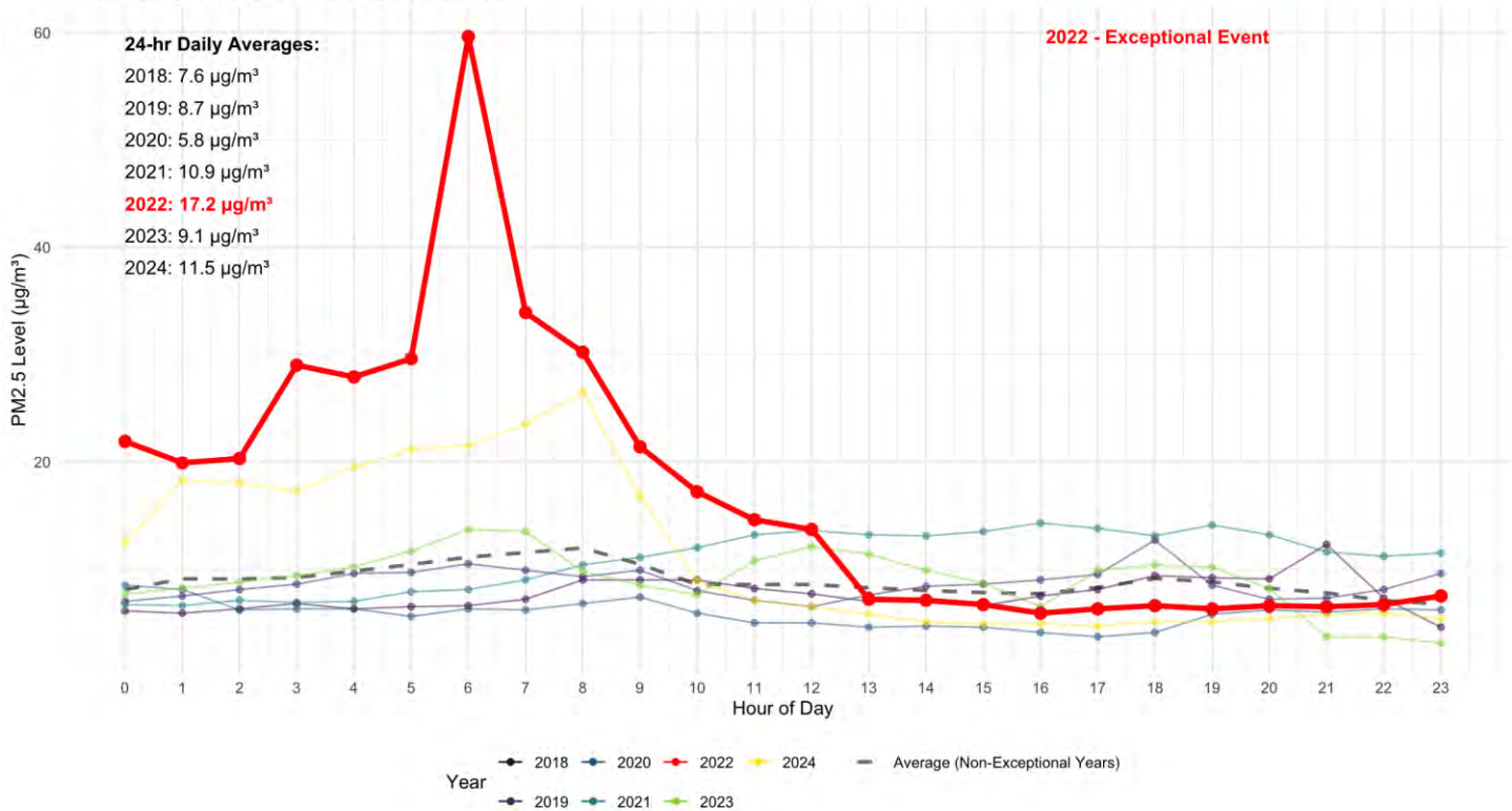
Hourly PM2.5 Levels on February 16th Across Years Forrest County - Exceptional Event Highlighted (2022)
