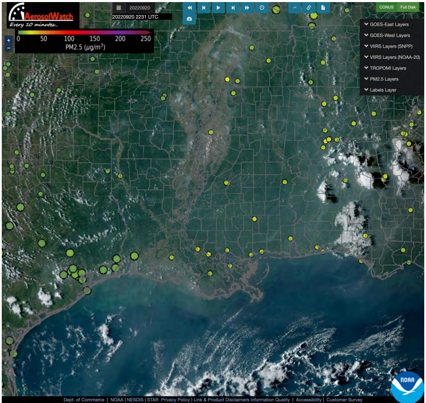
GOES True color imagery at 2231UTC (17:31CDT) showing smoke layer across Mississippi and Alabama, increasing PM2.5 Values.
