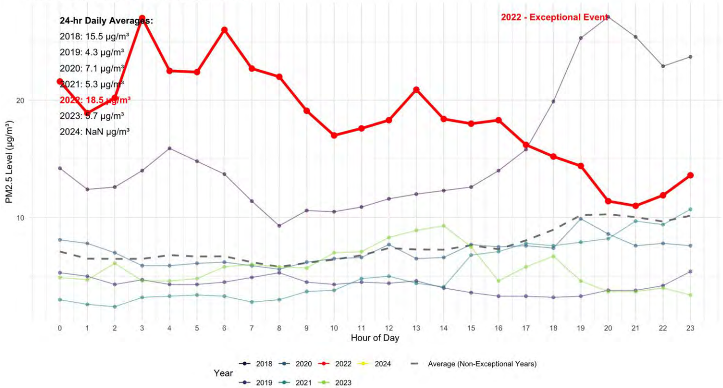
Hourly PM2.5 Levels on May 12th Across Years Forrest County - Exceptional Event Highlighted (2022)
