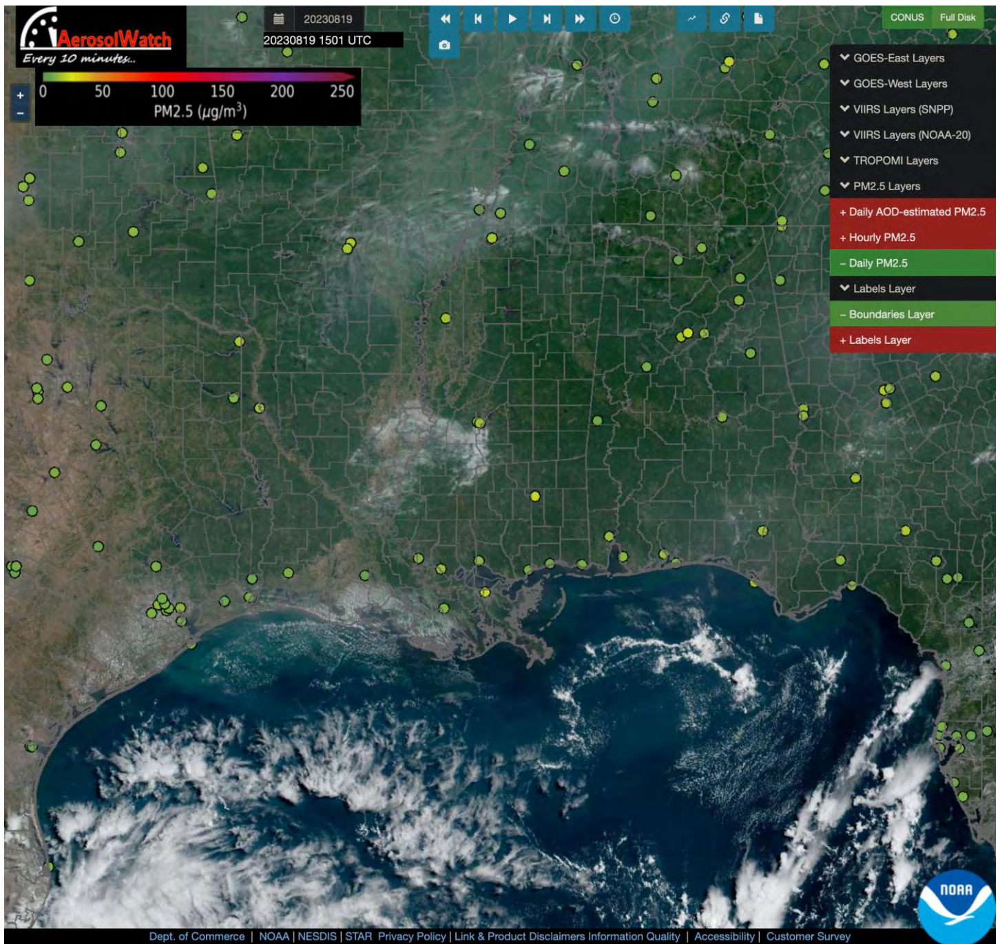
GOES East True Color image taken on August 19 th , 2023, at 1501UTC, showing smoke shield from Canadian wildfires encompassing most of the southeastern United States, elevating PM2.5 values.
