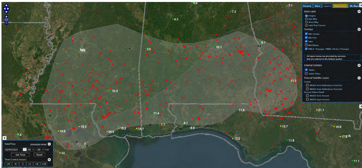
AirNowTech Navigator image above, showing the numerous ongoing prescribed fires in the southeast on March 4, 2023.
