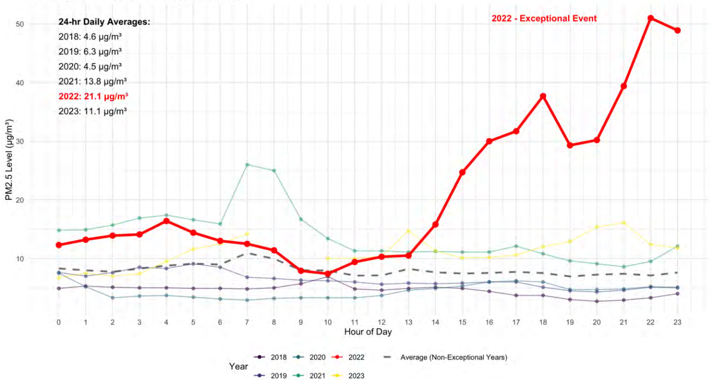
Hourly PM2.5 Levels on October 10th Across Years Forrest County - Exceptional Event Highlighted (2022)
