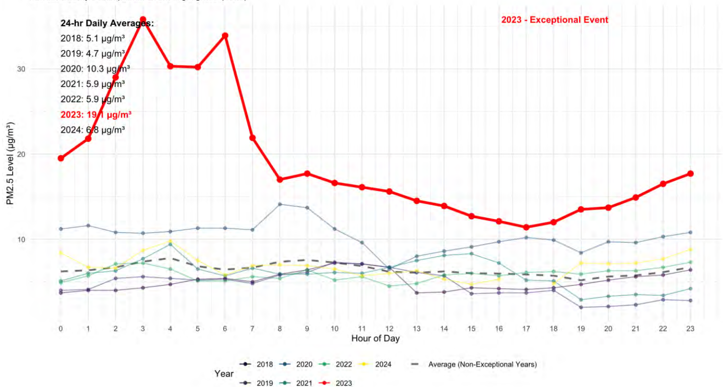
Hourly PM2.5 Levels on August 19th Across Years Forrest County - Exceptional Event Highlighted (2023)
