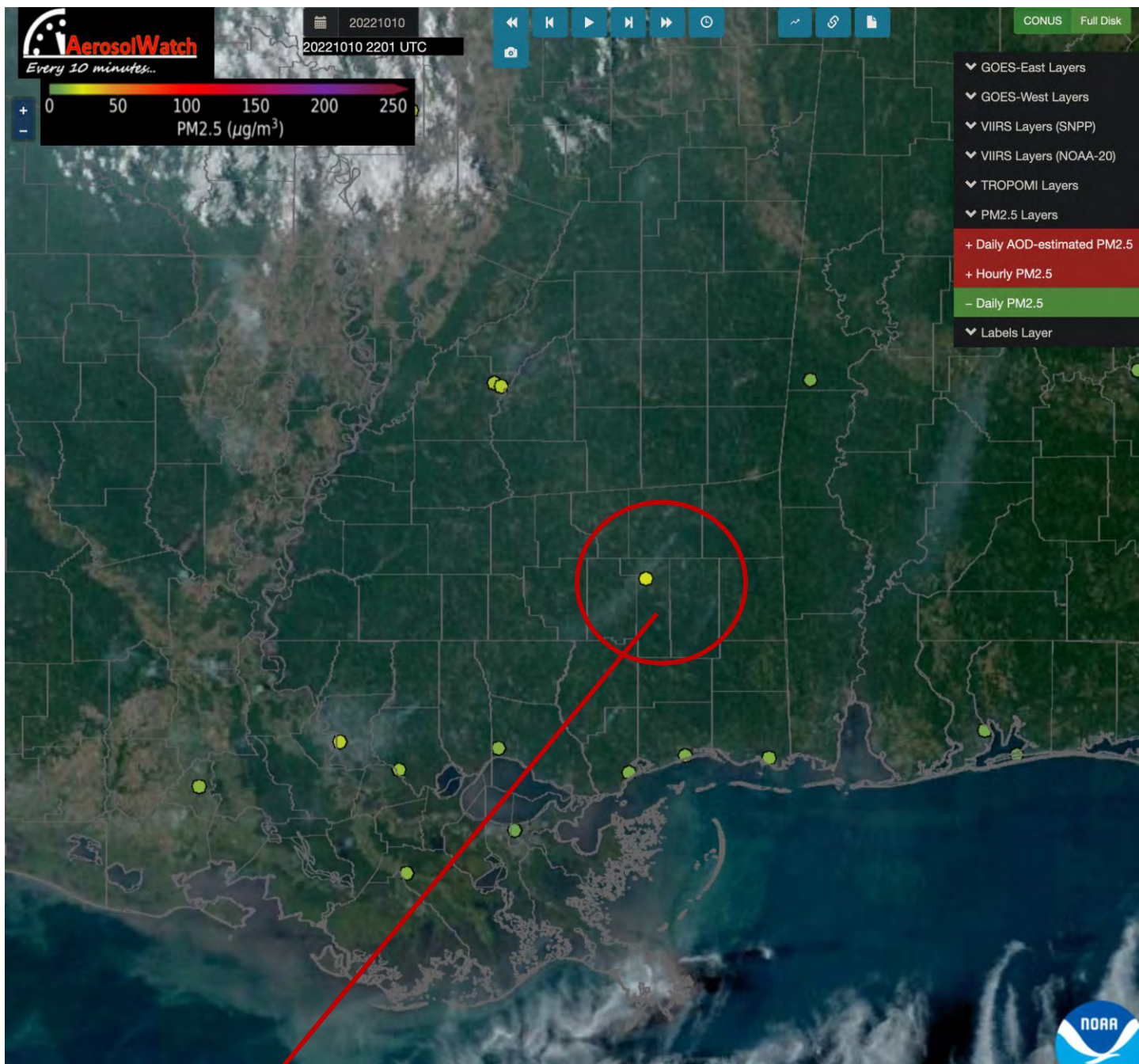
GOES True color imagery at 2201UTC (17:01CDT) showing smoke plume from prescribed fire in DeSoto National Forest affecting downwind Hattiesburg monitor as smoke was caught up in northeasterly wind flow.
